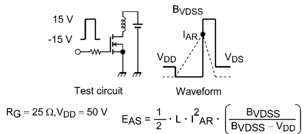
Fig. 8.16 Test Circuit/Waveform
