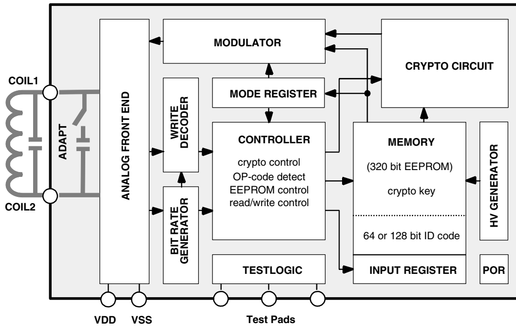
Figure 1-2. Block Diagram
