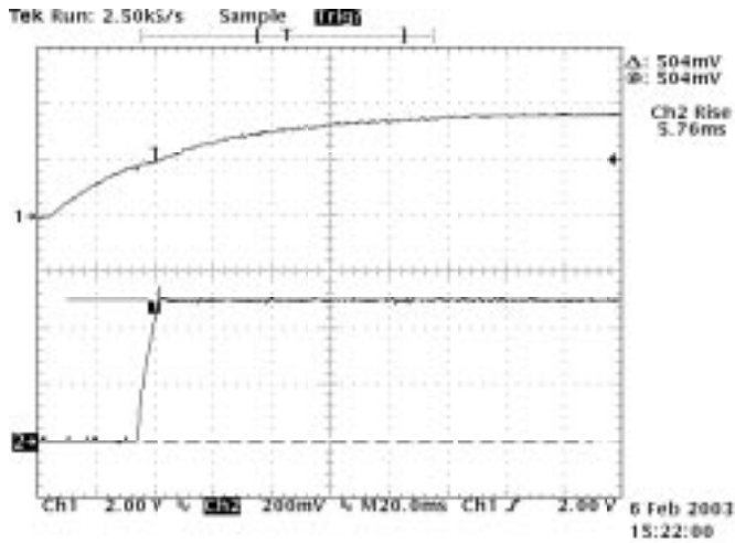
Channel 1 is Supply Voltage Channel 2 is the Feedback Voltage coming up to regulation.
