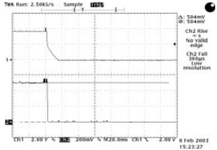
Channel 1 Supply Voltage turns off Channel 2 Feedback Voltage follows.
