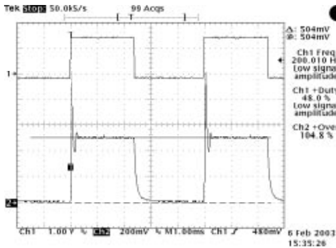
Channel 1 is the Enable waveform to create a change in intensity Channel 2 shows the Feedback Voltage reacting to the Enable signal.
