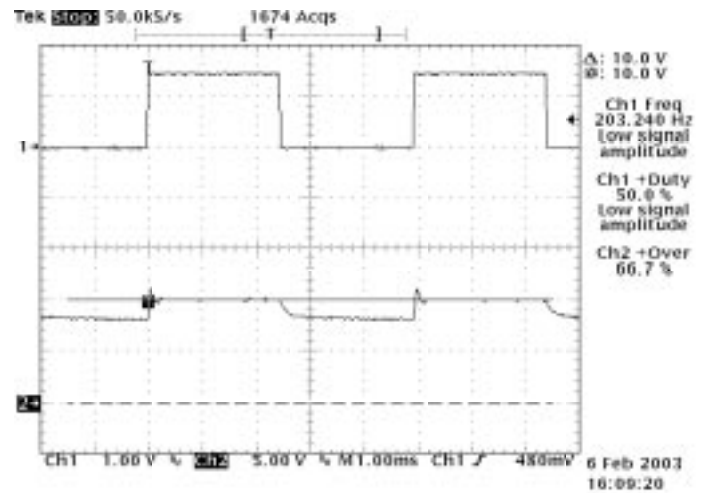
Channel 1 is the Enable waveform Channel 2 Output Voltage reacting to Enable signal
