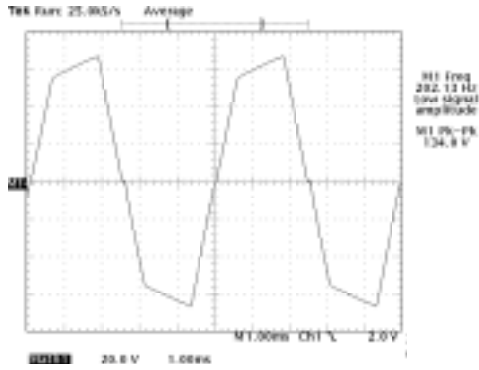
TK65921 Voltage Waveform Across 12 nF Lamp
