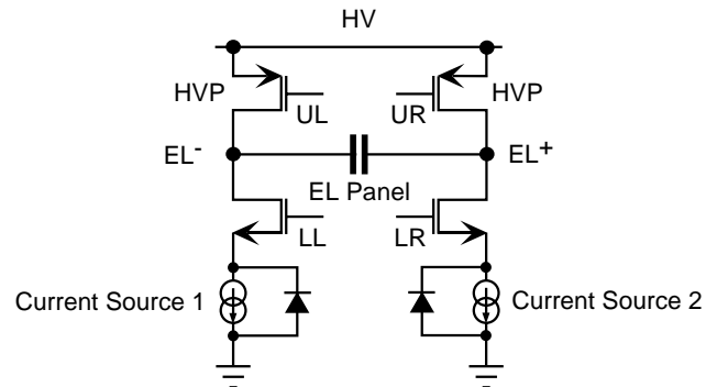
FIGURE 2: H-BRIDGE SCHEMATIC
