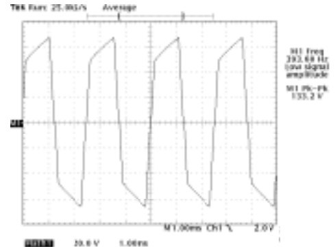
TK65929 Voltage Waveform Across 12 nF Lamp
