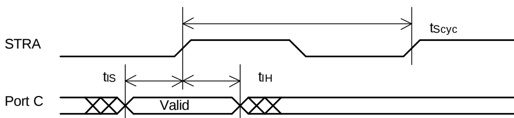
Figure 6. Simple Input Strobe Timing
