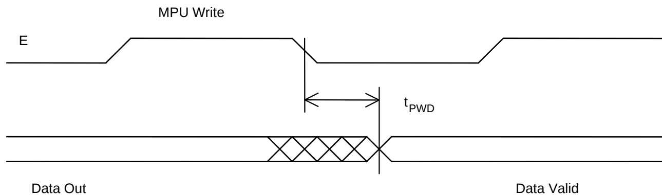
Figure 3. Port Write Timing
