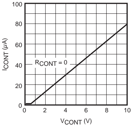
CONTROL CURRENT 1 vs. CONTROL VOLTAGE
