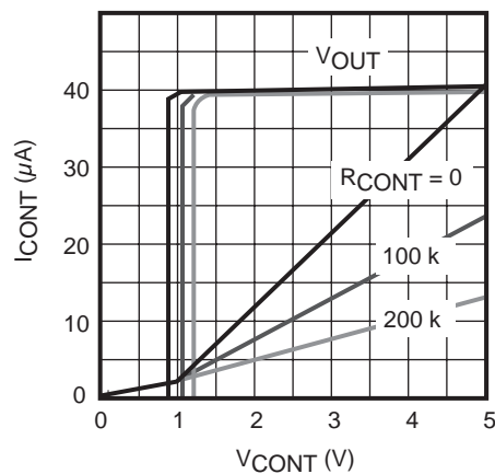
CONTROL CURRENT 2 vs. CONTROL VOLTAGE
