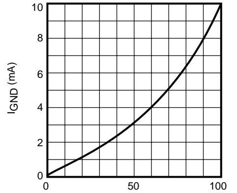
GROUND CURRENT vs. OUTPUT CURRENT
