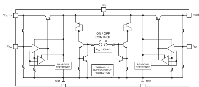
BLOCK DIAGRAM
