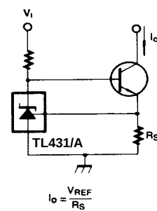
Figure 14. Constant-Current Sink
