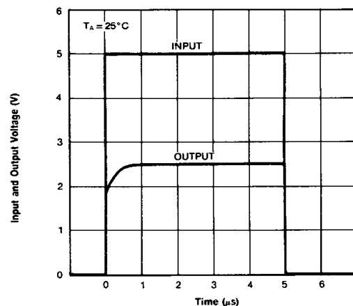
Figure 6. Pulse Response
