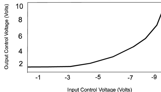
Output Control Voltage vs. Input Voltage
