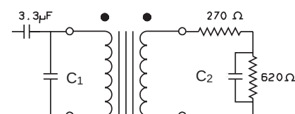
Fig.2: Test circuit
