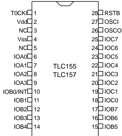
PDIP, SOP
