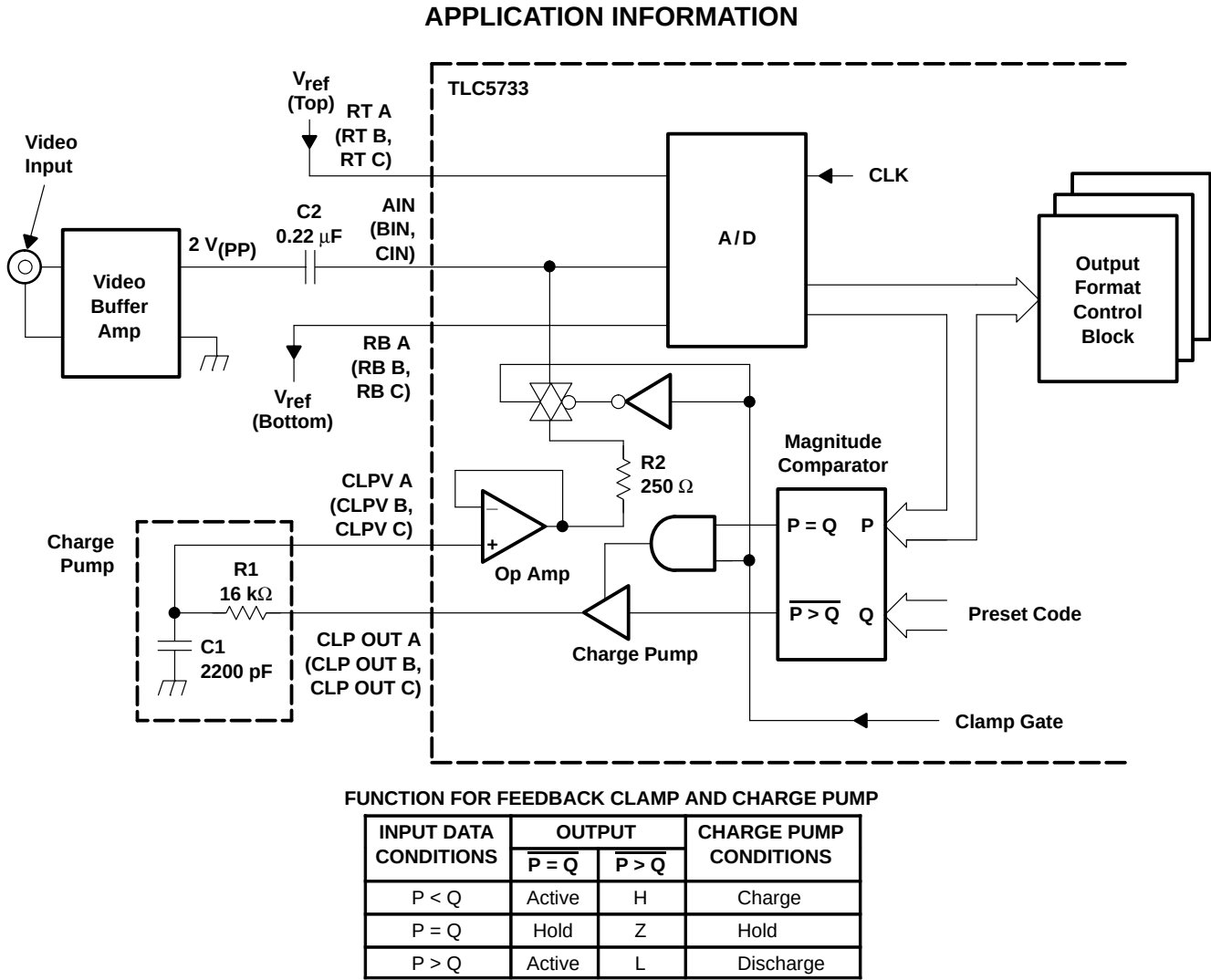
Figure 6. Feedback Clamp Circuit
