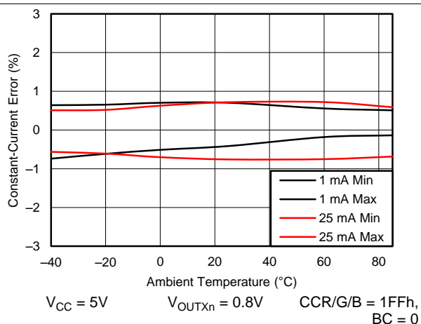
Figure 5. Constant-Current Error (CH-to-CH) vs Temperature
