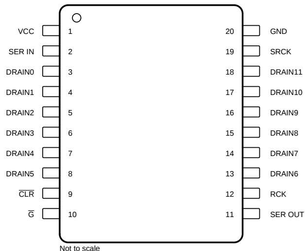
PW Package 20-Pin TSSOP Top View
