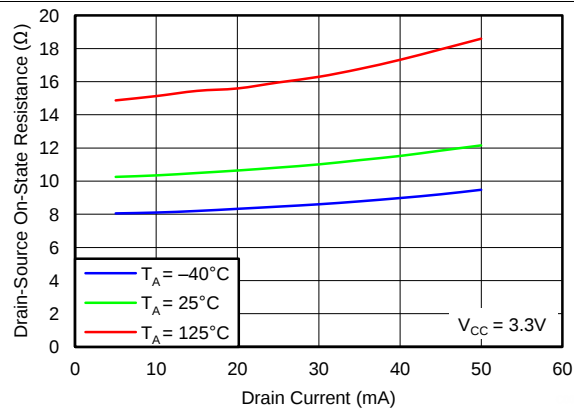
Figure 6. Drain-to-Source On-State Resistance vs Drain Current
