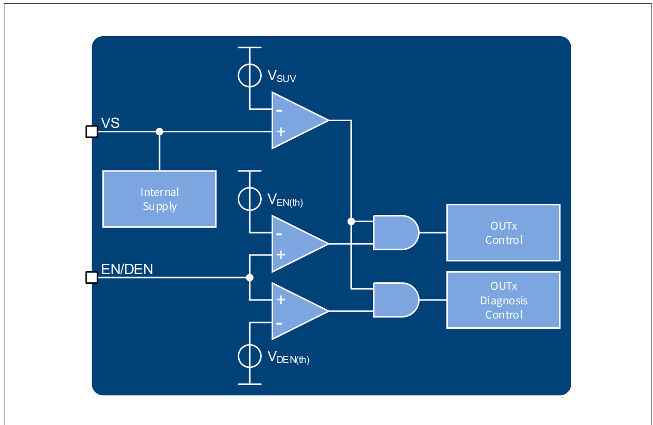
Figure 3 Internal supply
