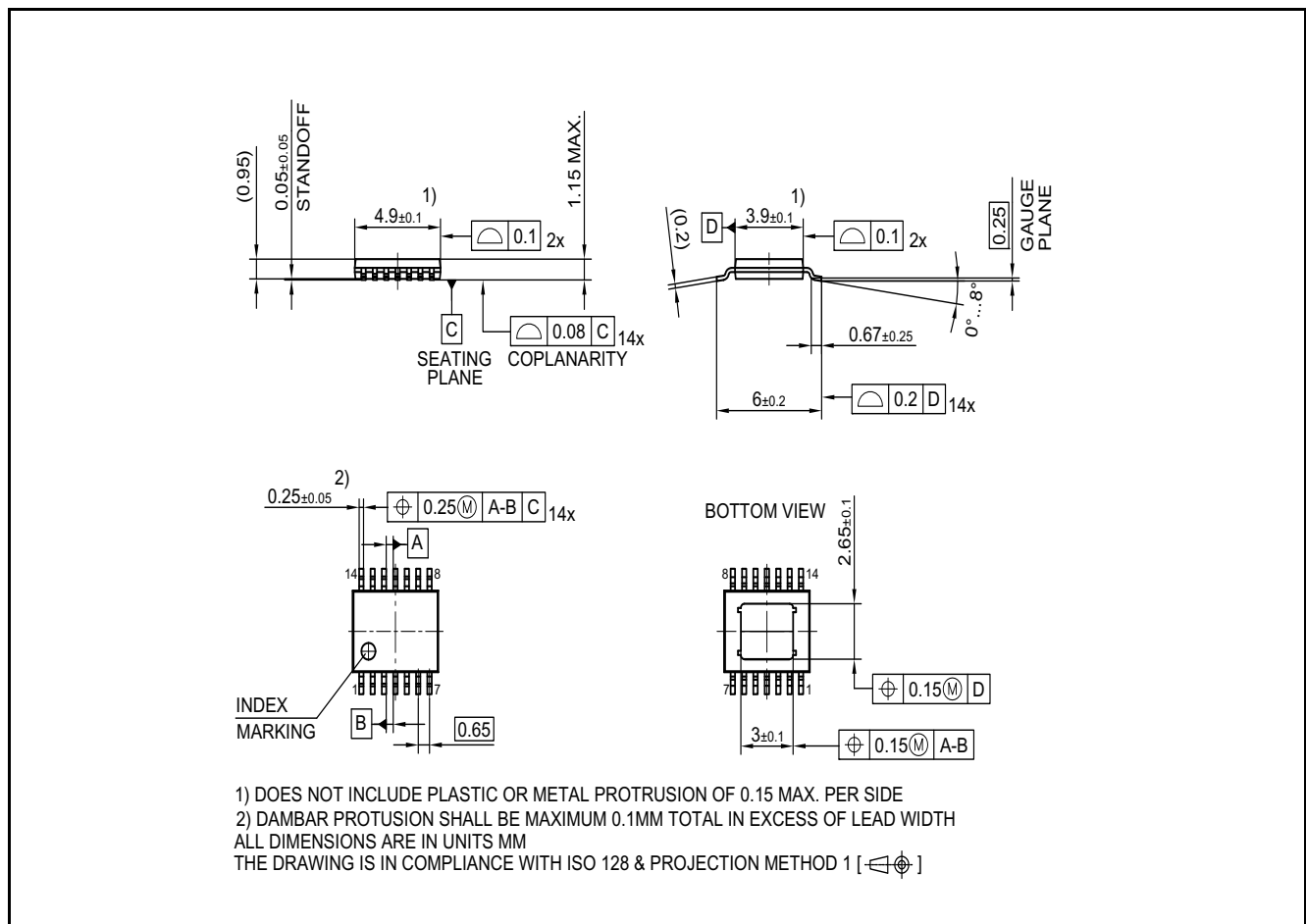
Figure 32 Outline PG-TSDSO-14
