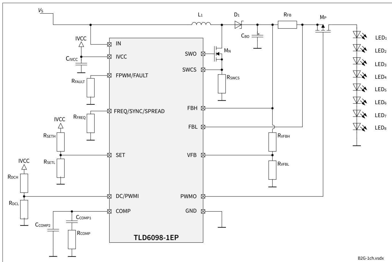
Figure 1 Application diagram
