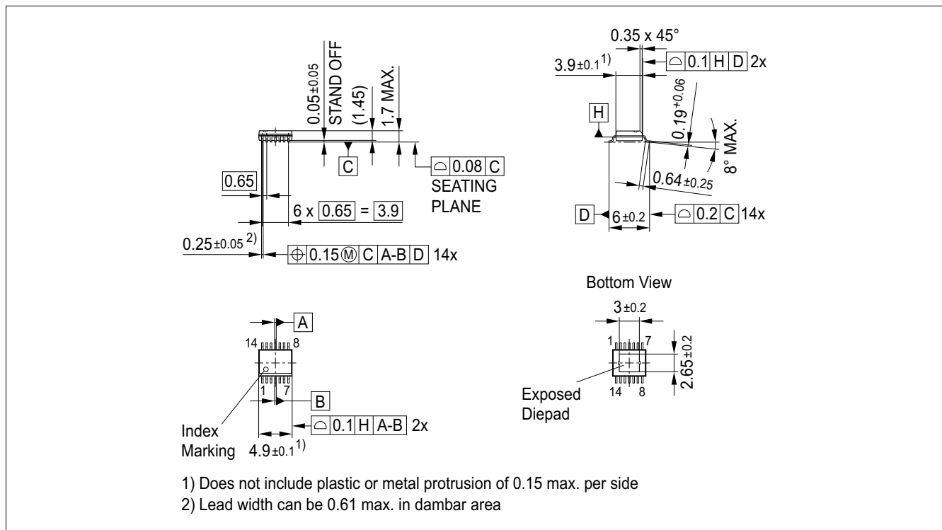
Figure 4 PG-SSOP-14 exposed pad 1)
