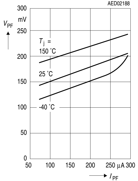
Power Fail Low Voltage V_{PF} versus Power Fail Current I_{PF}
