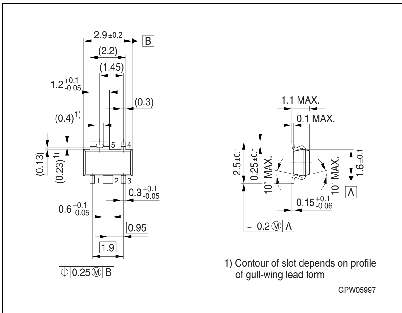
Figure 4 Outline PG-SCT595-5
