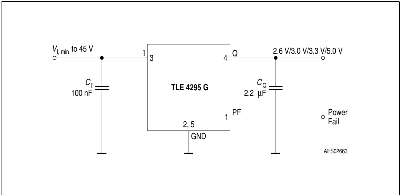
Figure 3 Application Circuit
