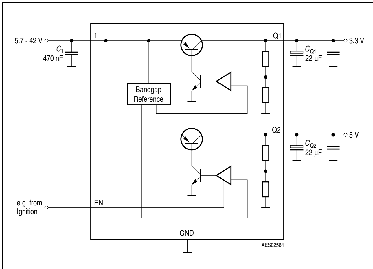
Figure 3 Application Circuit
