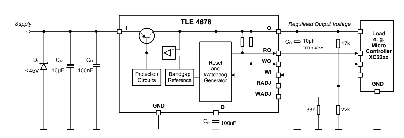
Figure 14 Application Diagram with Reset and Watchdog activation Threshold Adjustment
