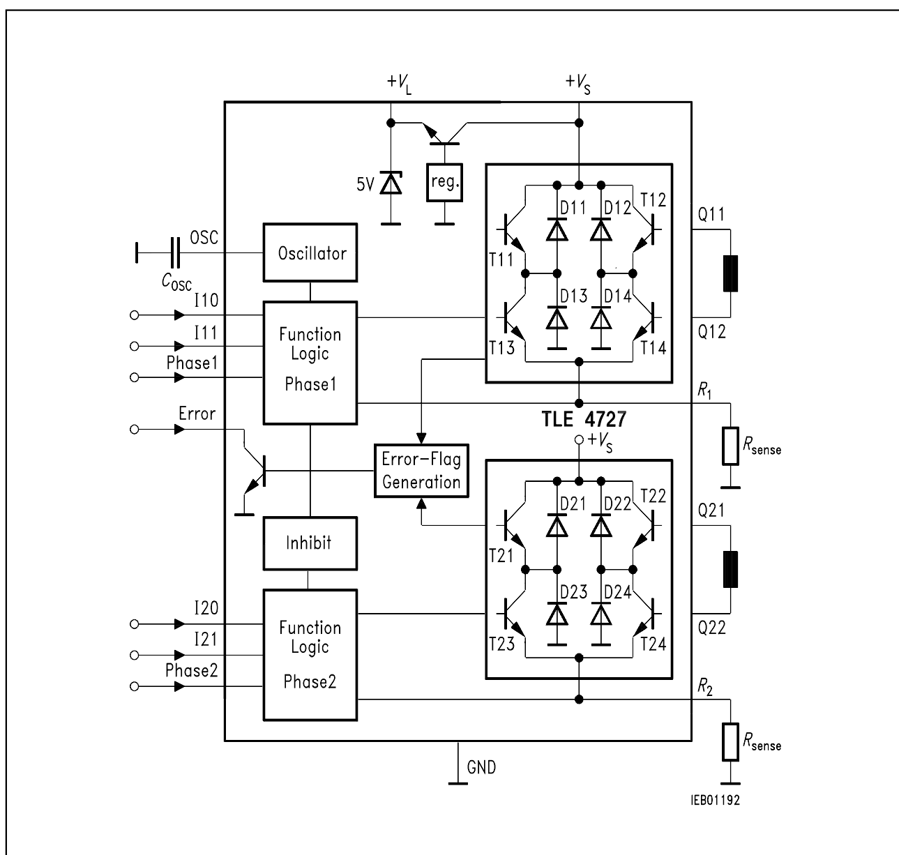
Figure 2 Block Diagram
