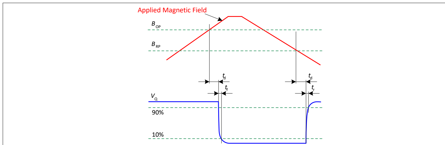
Figure 5 Timing diagram
