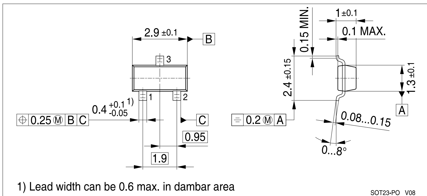
Figure 17 Outline of package SOT23-3 with dimensions
