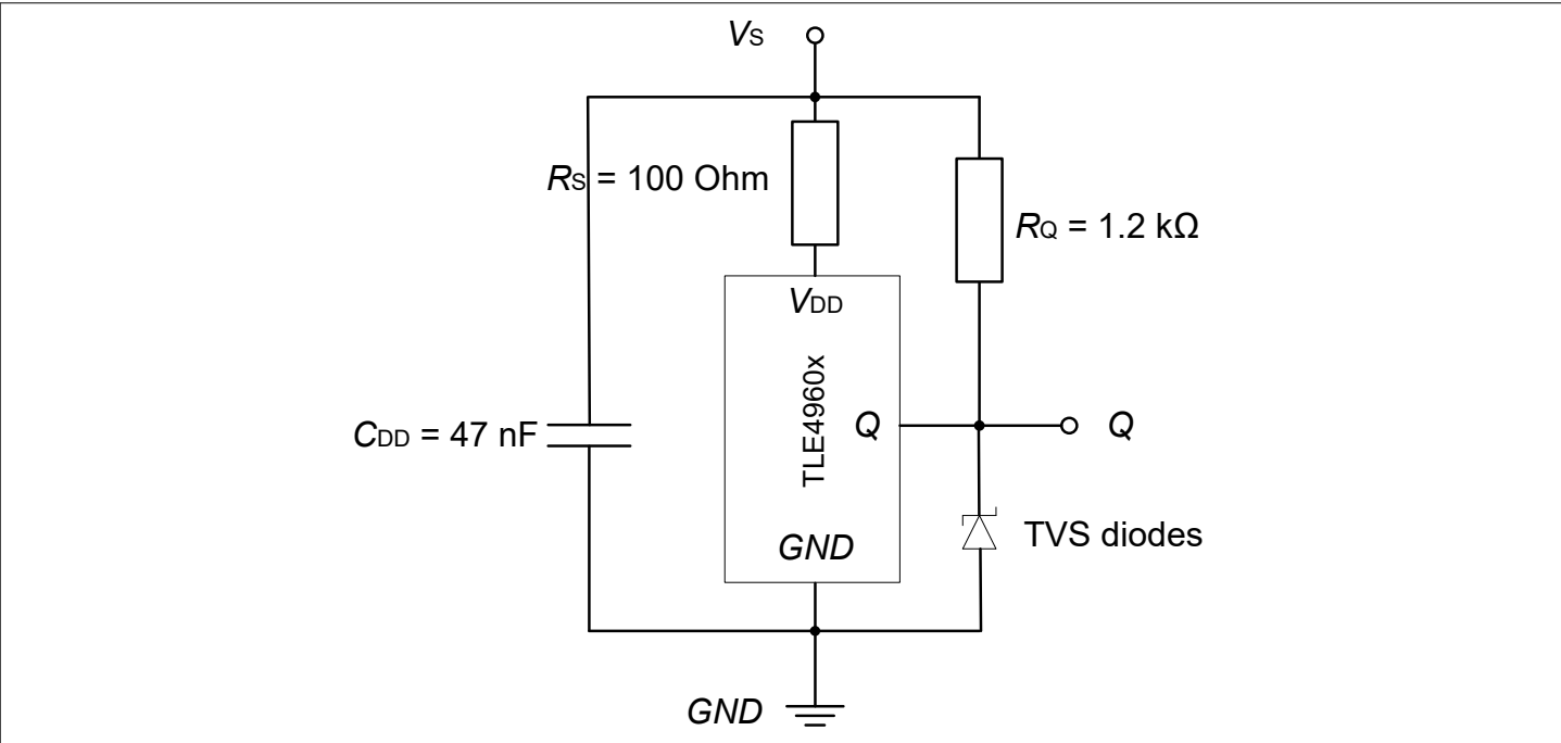
Figure 14 Application circuitry for harsh environmental conditions
