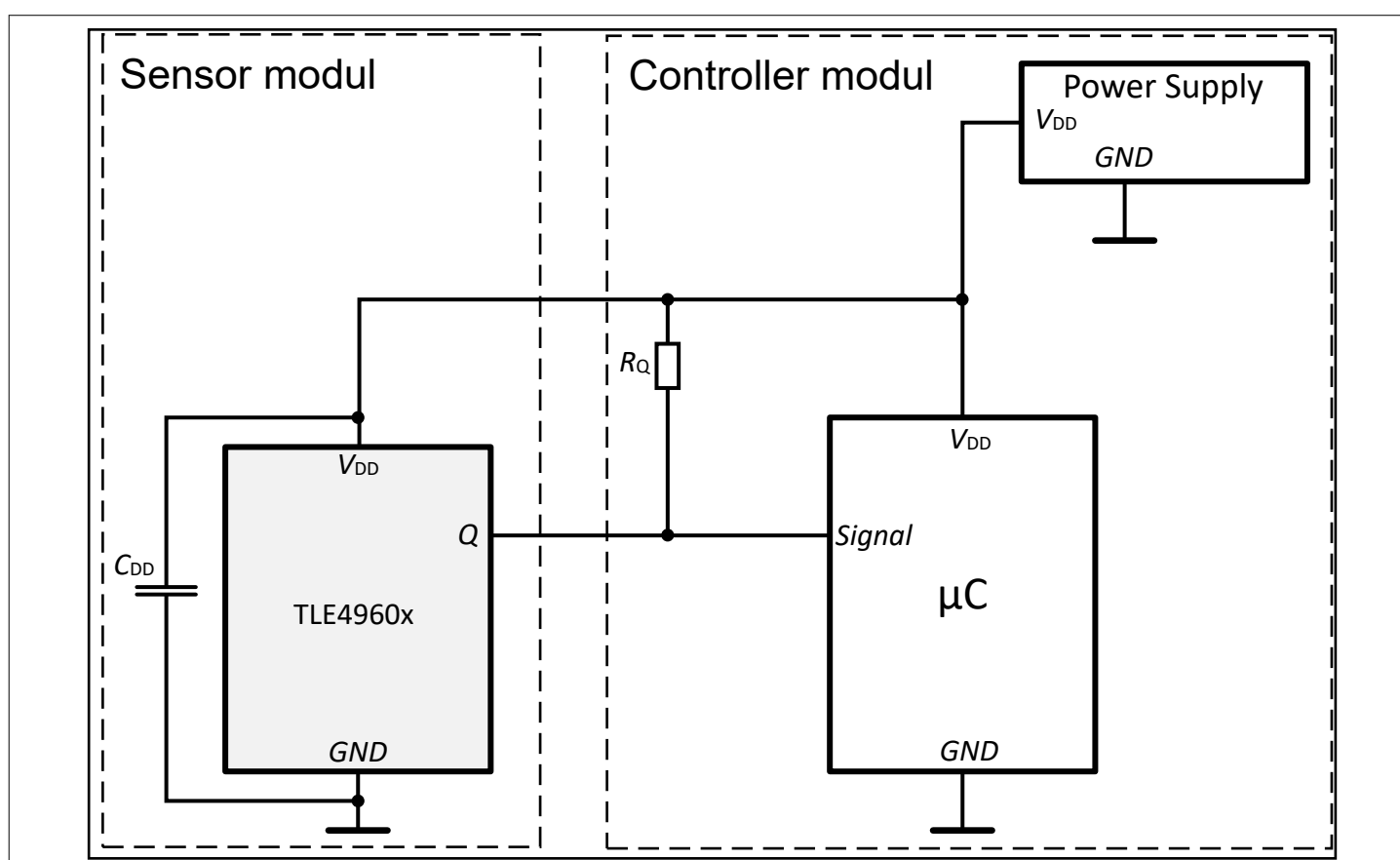
Figure 12 Example application diagram in 3-wire configuration
