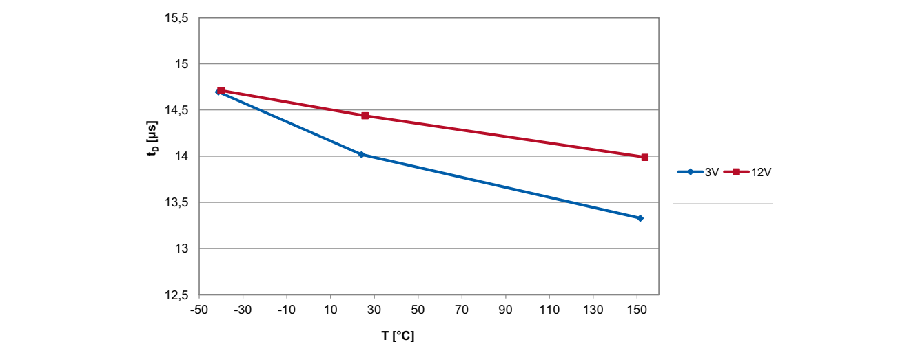
Figure 6-2 Signal Delay Time of the TLE4968-1K over Temperature
