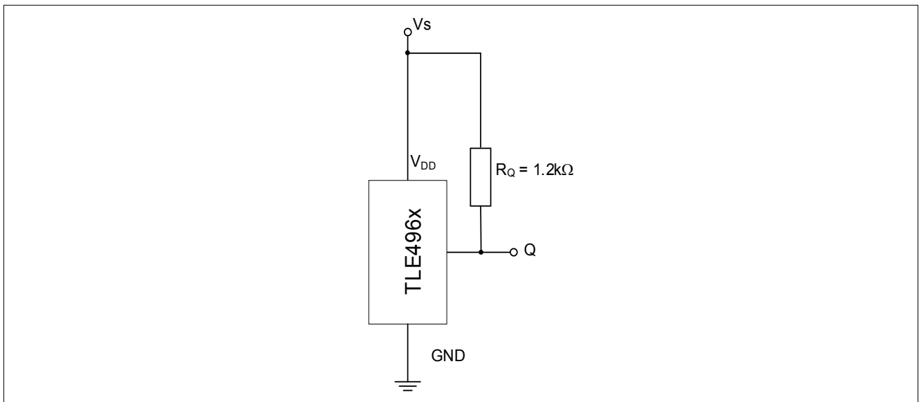
Figure 3-1 Basic Application Circuit #1: Only Pull-Up Resistor is necessary
