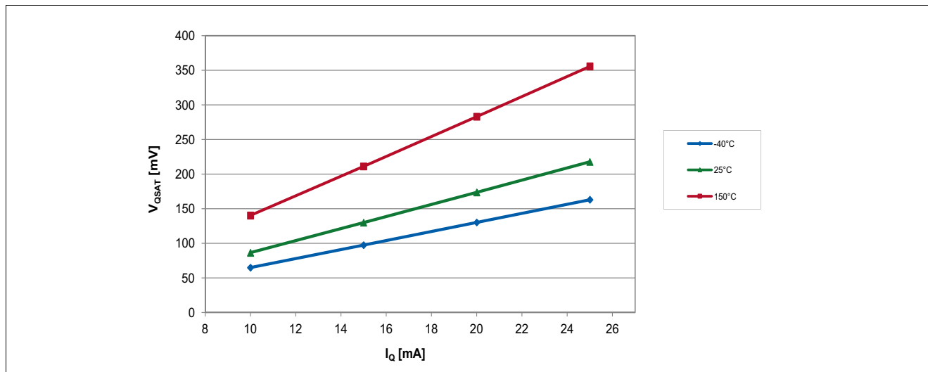
Figure 6-13 Saturation Voltage of the TLE4968-1M over Output Current
