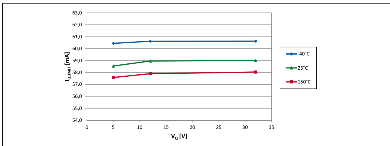
Figure 6-6 Output Current Limit of the TLE4968-1M over applied Pull-up Voltage
