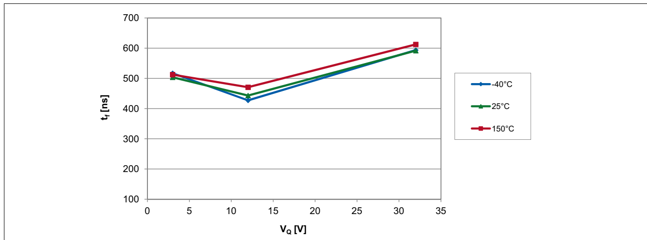
Figure 6-10 Output Rise Time of the TLE4968-1M over applied Pull-up Voltage
