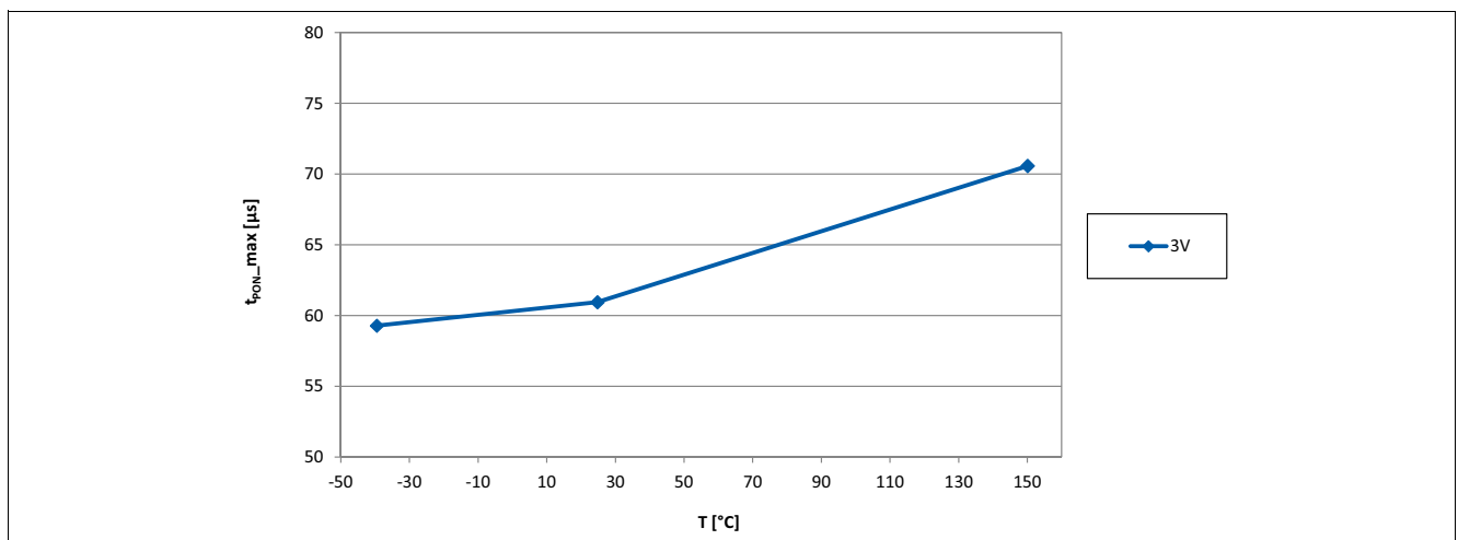
Figure 6-1 Power On Time t_{PON} of the TLE4968-1M over Temperature
