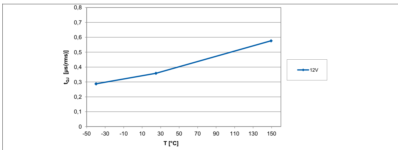
Figure 6-15 Output Signal Jitter of the TLE4968-1M over Temperature
