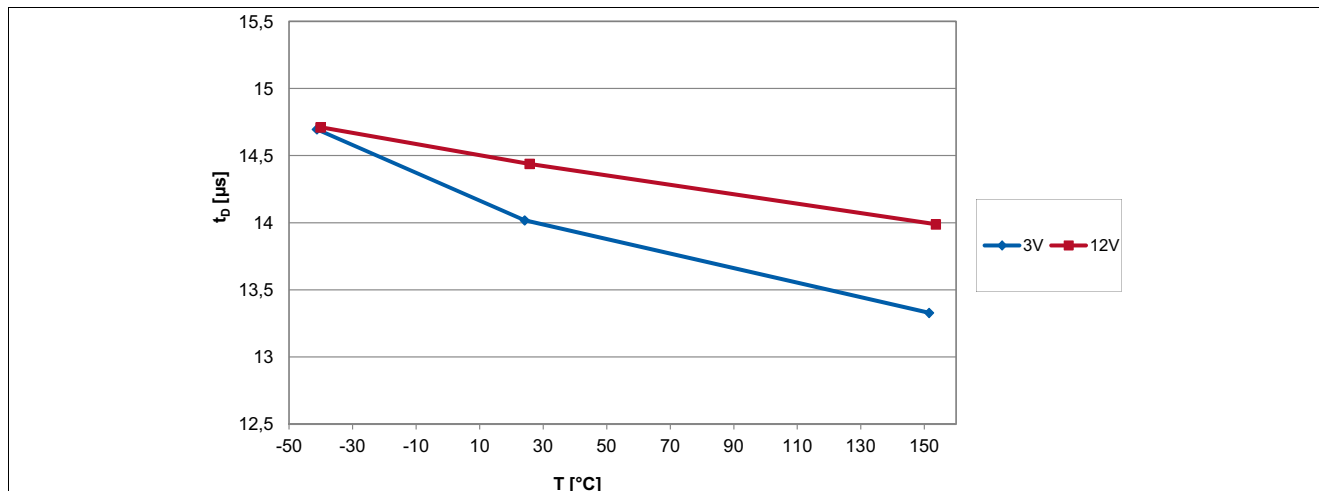
Figure 6-2 Signal Delay Time of the TLE4968-1M over Temperature
