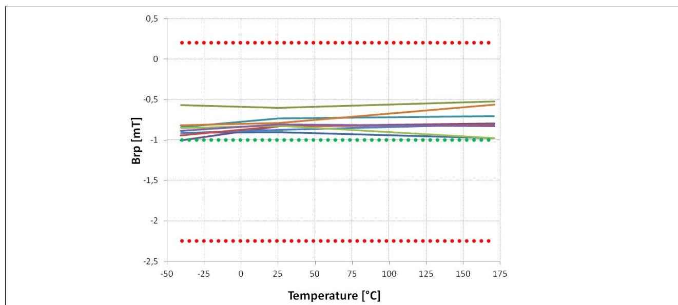
Figure 5-2 Release Point ( B_{RP} ) of the TLE4968-1M over Temperature
