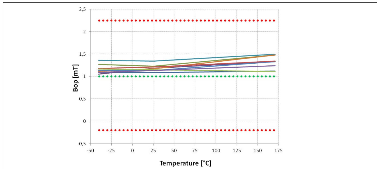
Figure 5-1 Operating Point ( B_{OP} ) of the TLE4968-1M over Temperature
