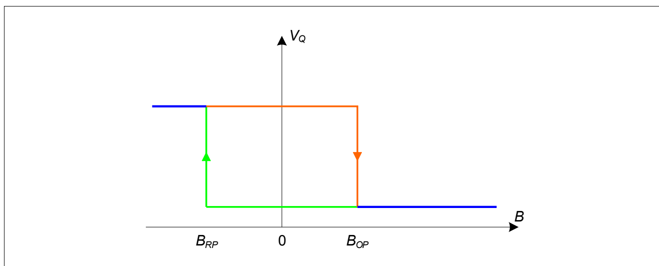
Figure 2-4 Output Signal TLE4968-1M
