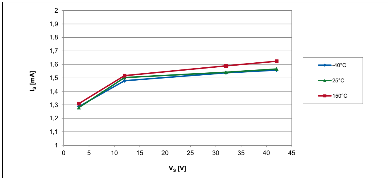
Figure 6-4 Supply Current of the TLE4968-1M over Supply Voltage
