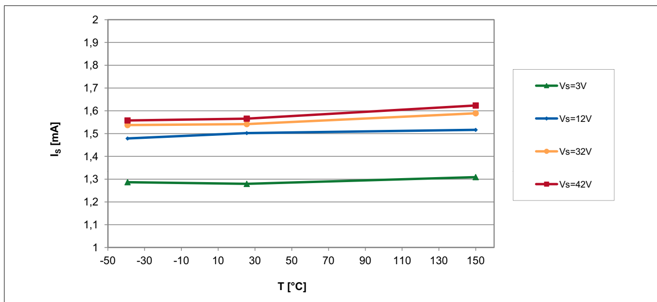
Figure 6-3 Supply Current of the TLE4968-1M over Temperature
