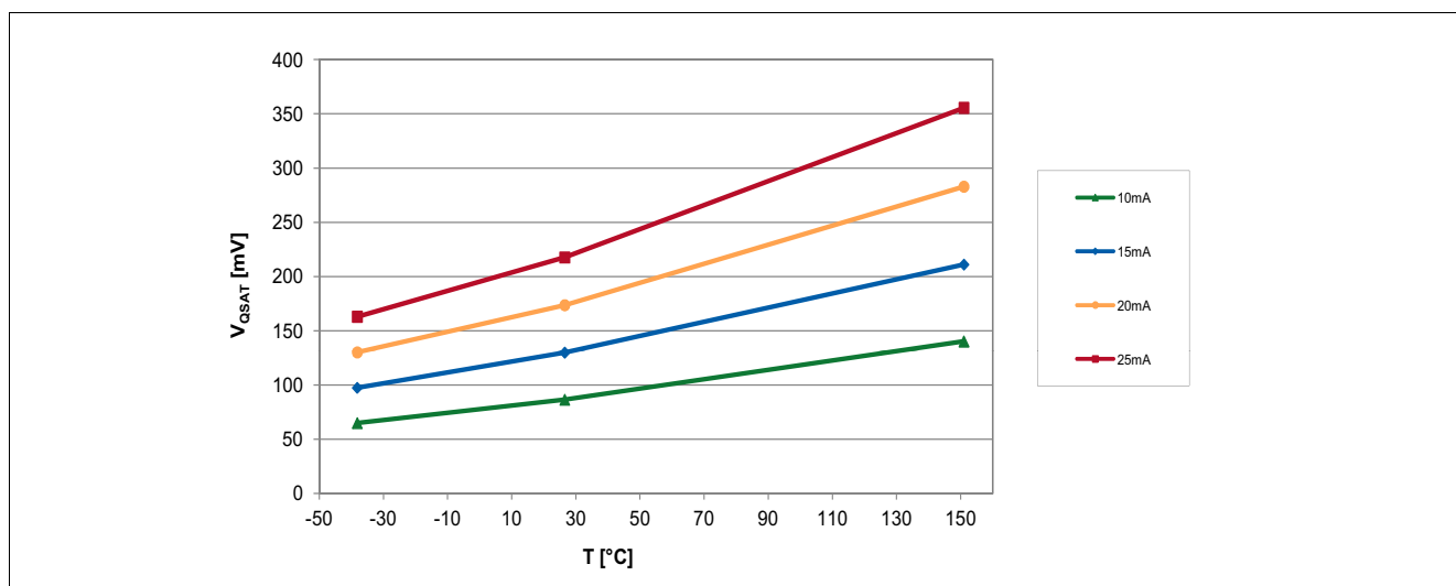
Figure 6-12 Saturation Voltage of the TLE4968-1M over Temperature
