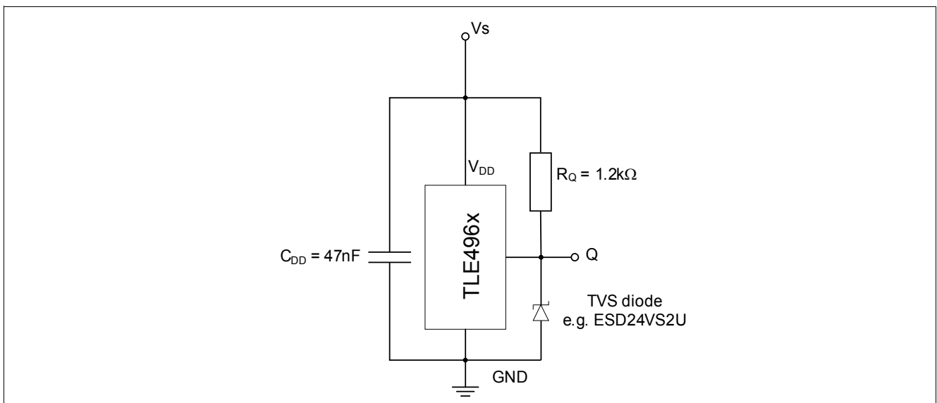
Figure 3-2 Enhanced Application Circuit #2 for extended ESD robustness
