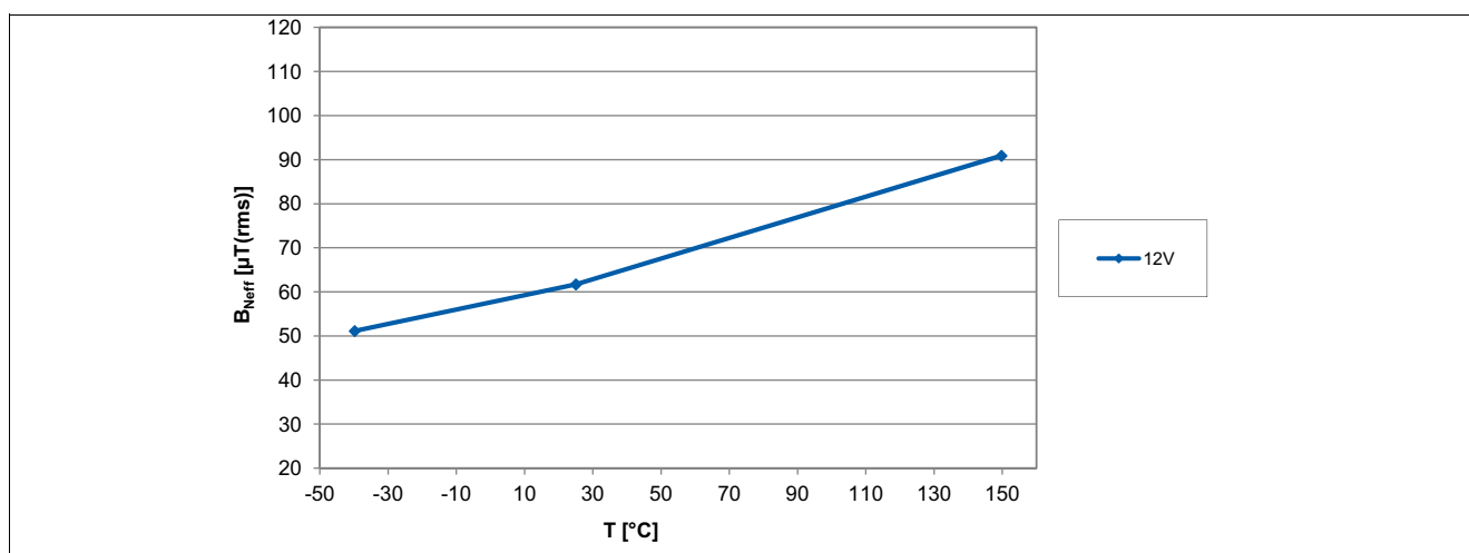
Figure 6-14 Effective Noise of the TLE4968-1M Thresholds over Temperature
