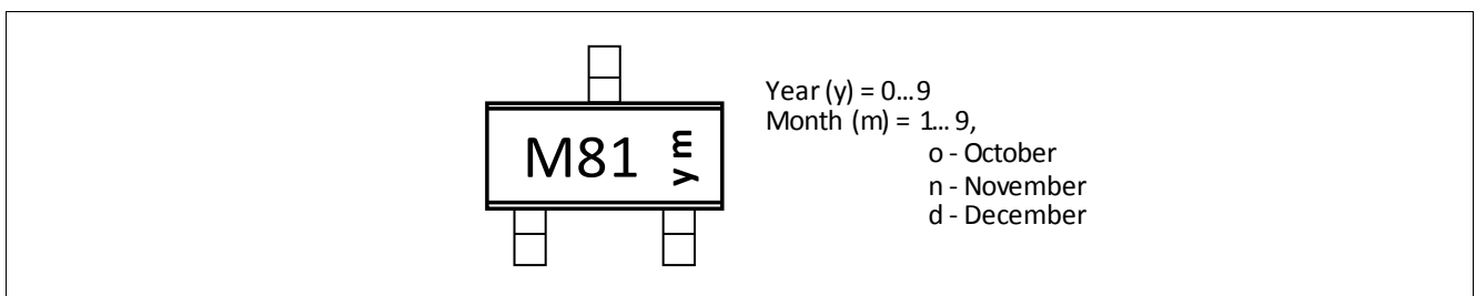
Figure 4-5 Marking of TLE4968-1M
