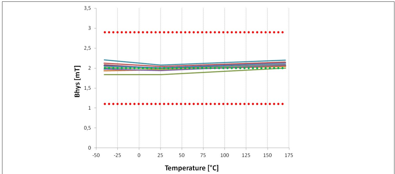
Figure 5-3 Hysteresis ( B_{Hys} ) of the TLE4968-1M over Temperature
