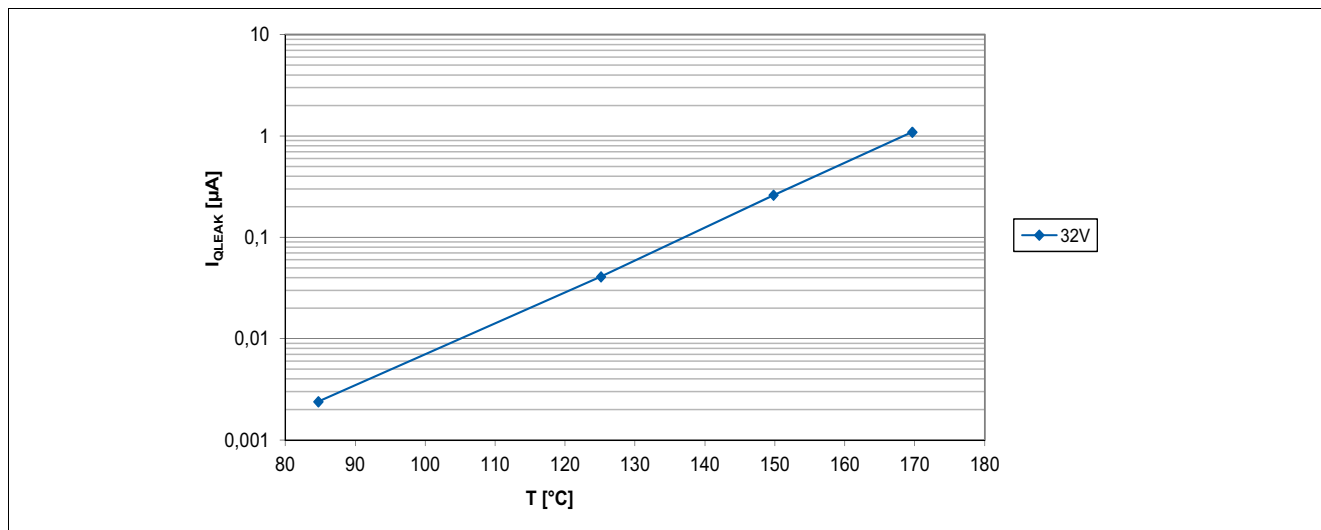
Figure 6-11 Output Leakage Current of the TLE4968-1M over Temperature
