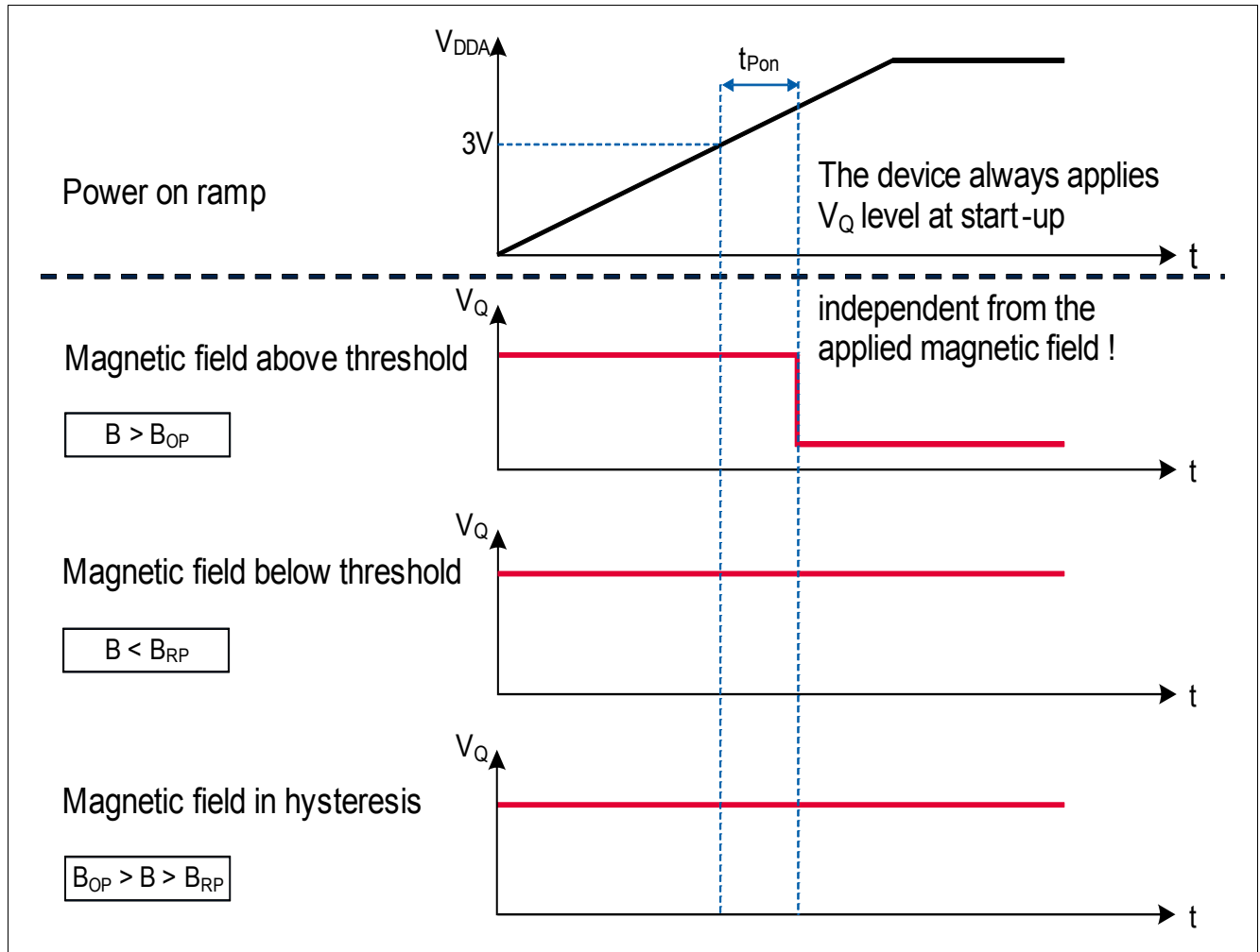
Figure 2-5 Illustration of the Start-up Behavior of the TLE4968-1M
