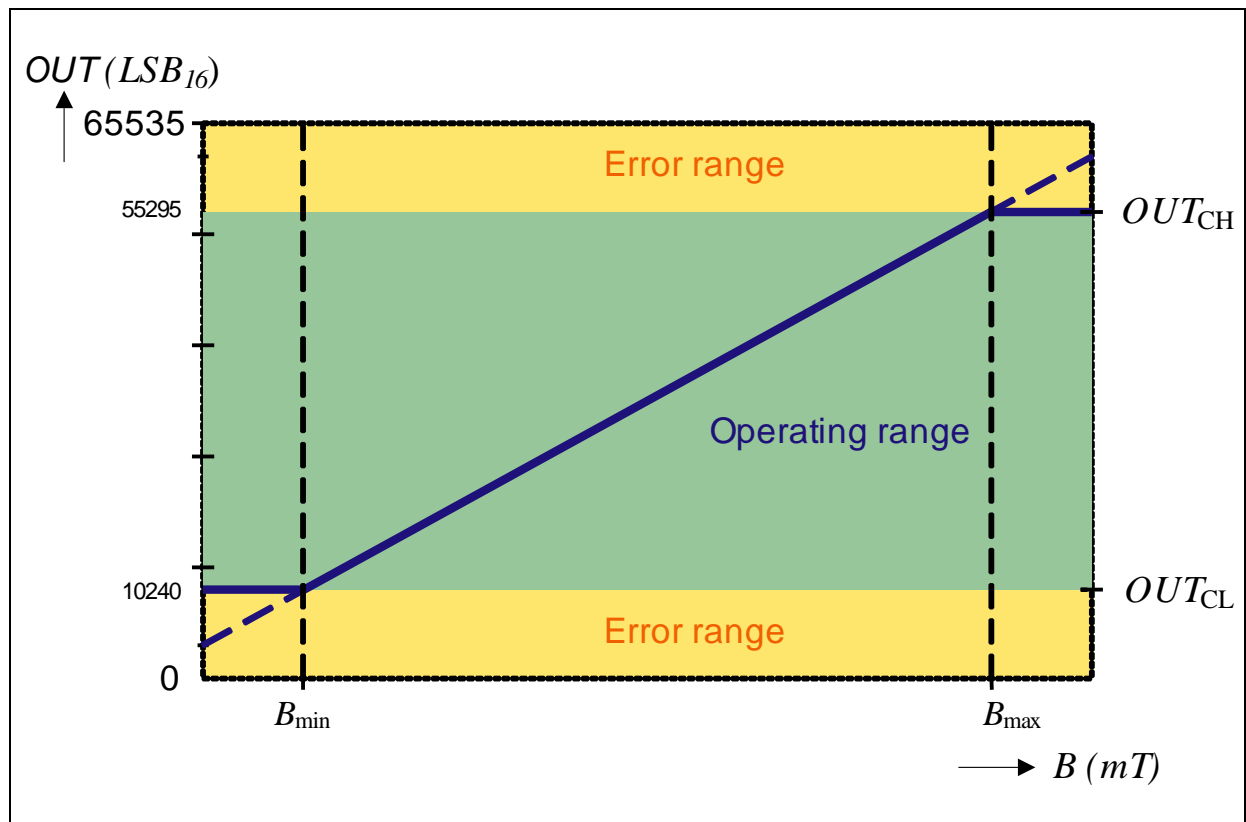
Figure 8 Clamping Example
