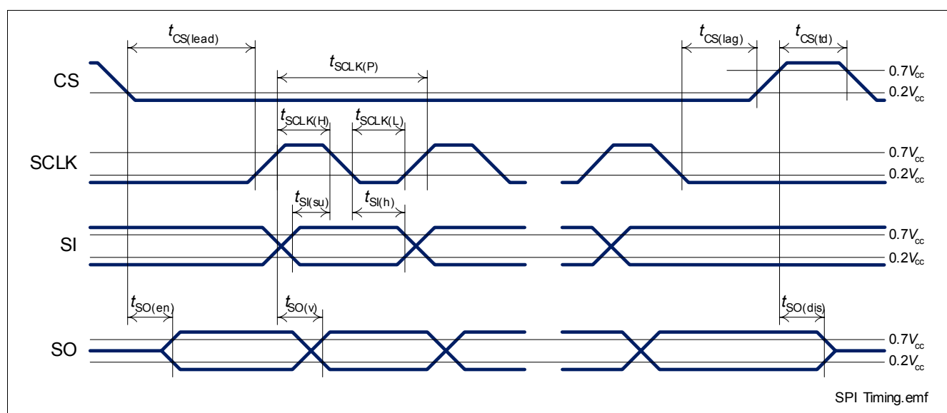
Figure 12 Timing Diagram
