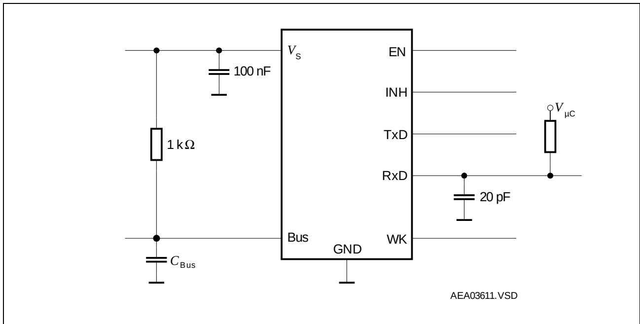
Figure 4 Test Circuits
