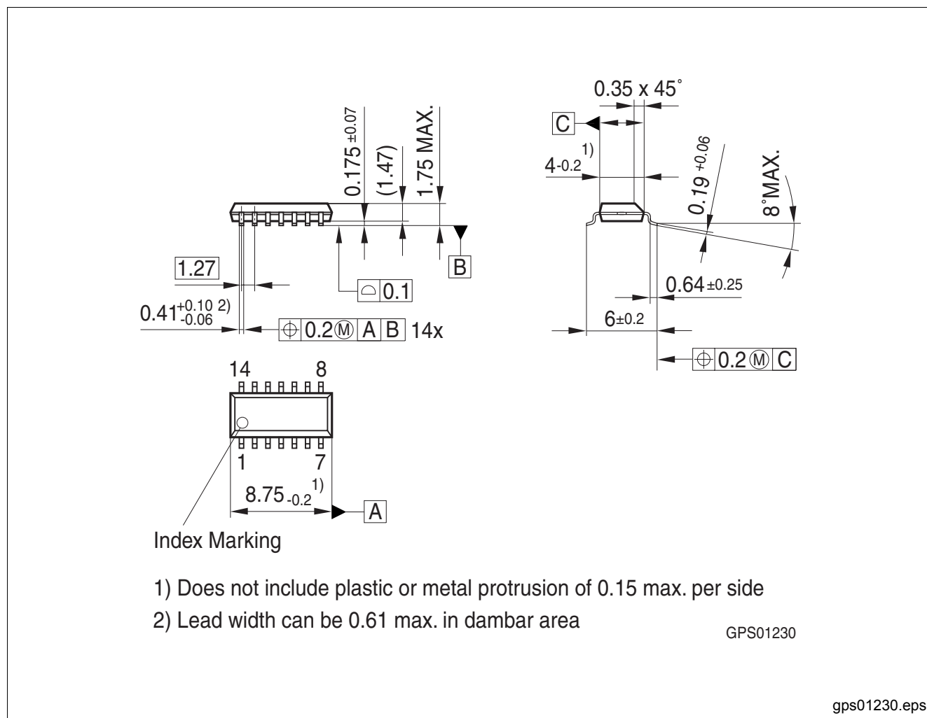
Figure 8 PG-DSO-14
