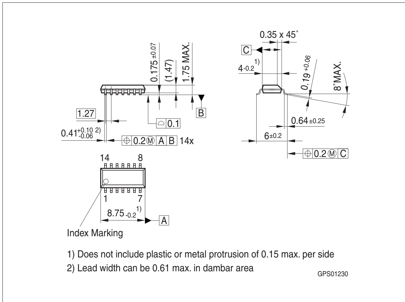
Figure 6 PG-DSO-14 (Plastic/Plastic Green - Dual Small Outline Package)
