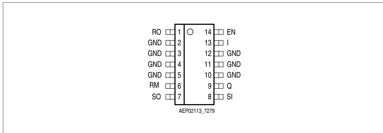
Figure 1 Pin Configuration
