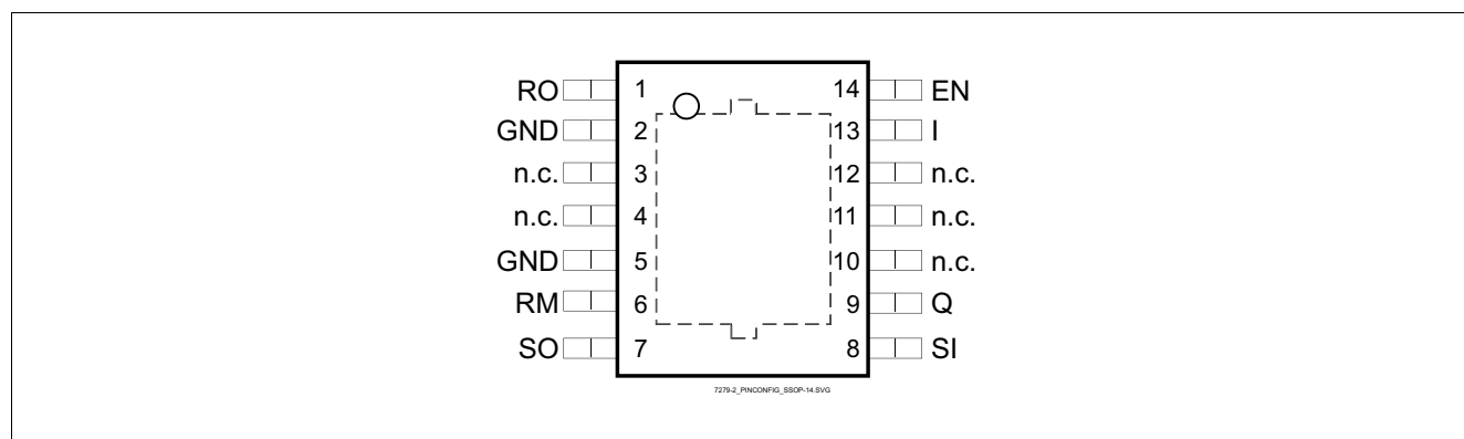
Figure 2 Pin Configuration
