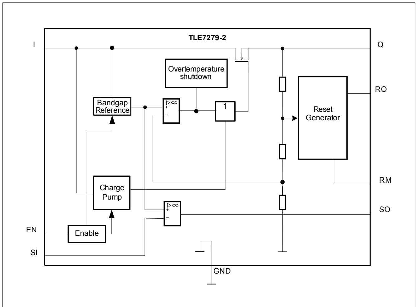
Figure 3 Block Diagram
