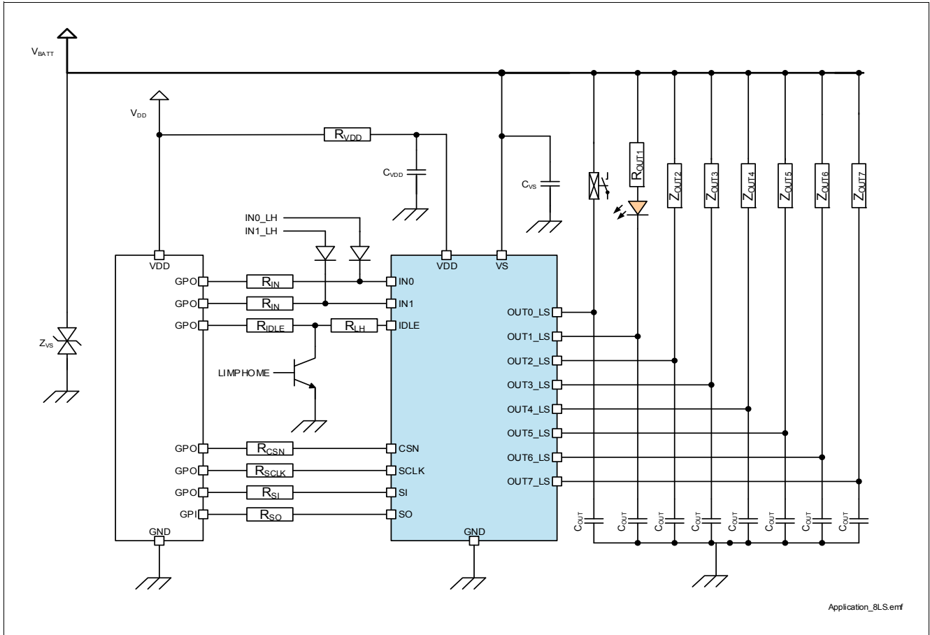
Figure 32 TLE75008-EMD Application Diagram
