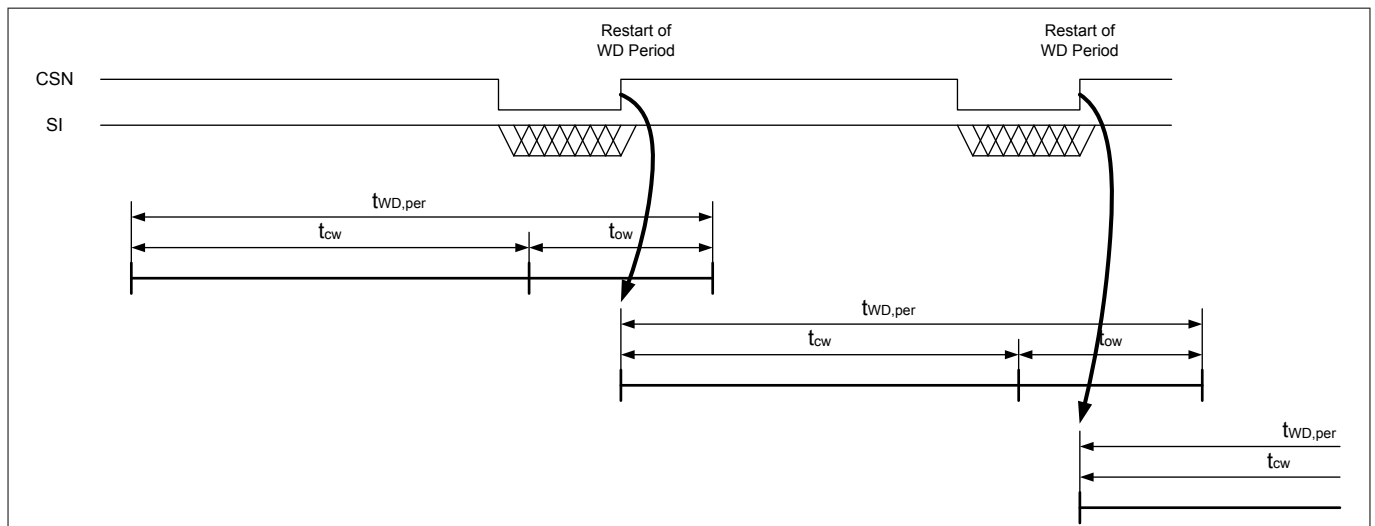
Figure 7 Watchdog trigger
