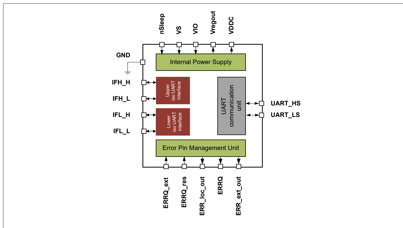
Figure 1 Block diagram
