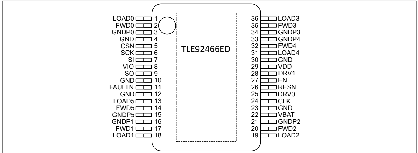
Figure 2 Pin assignment
