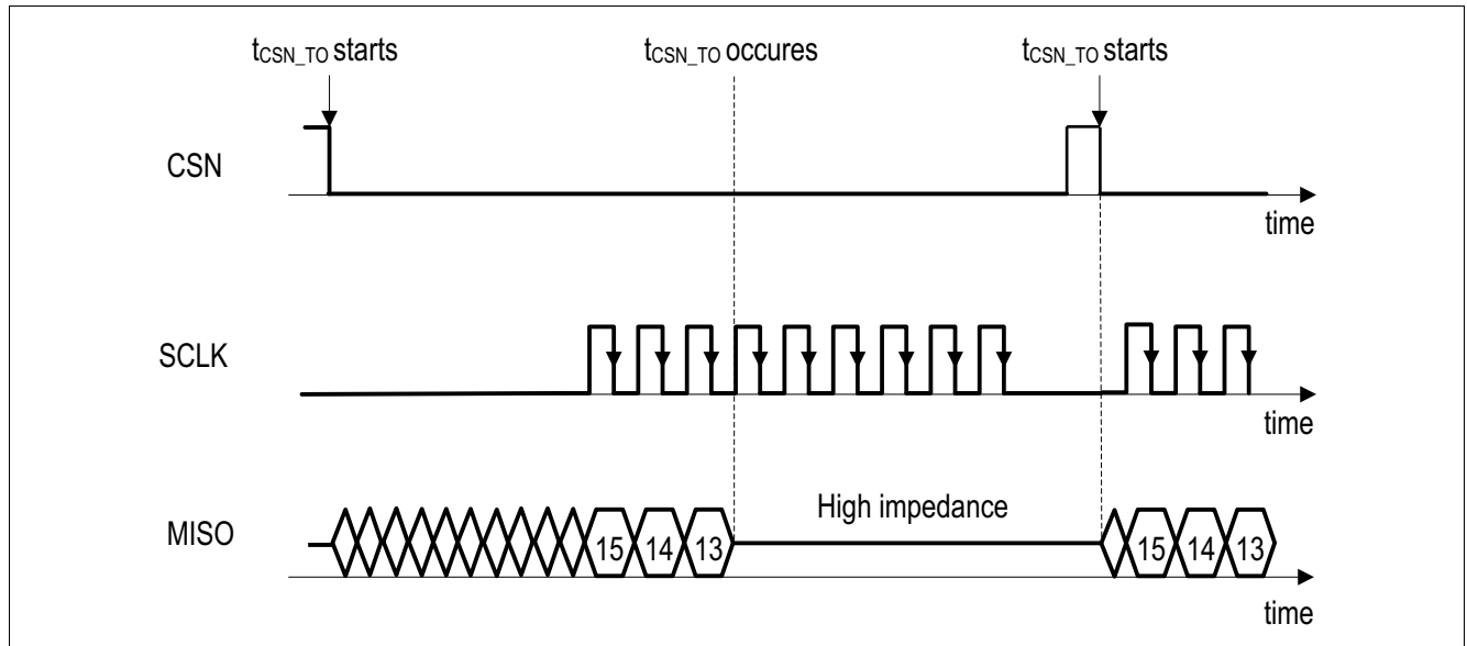
Figure 45 CSN Timeout
