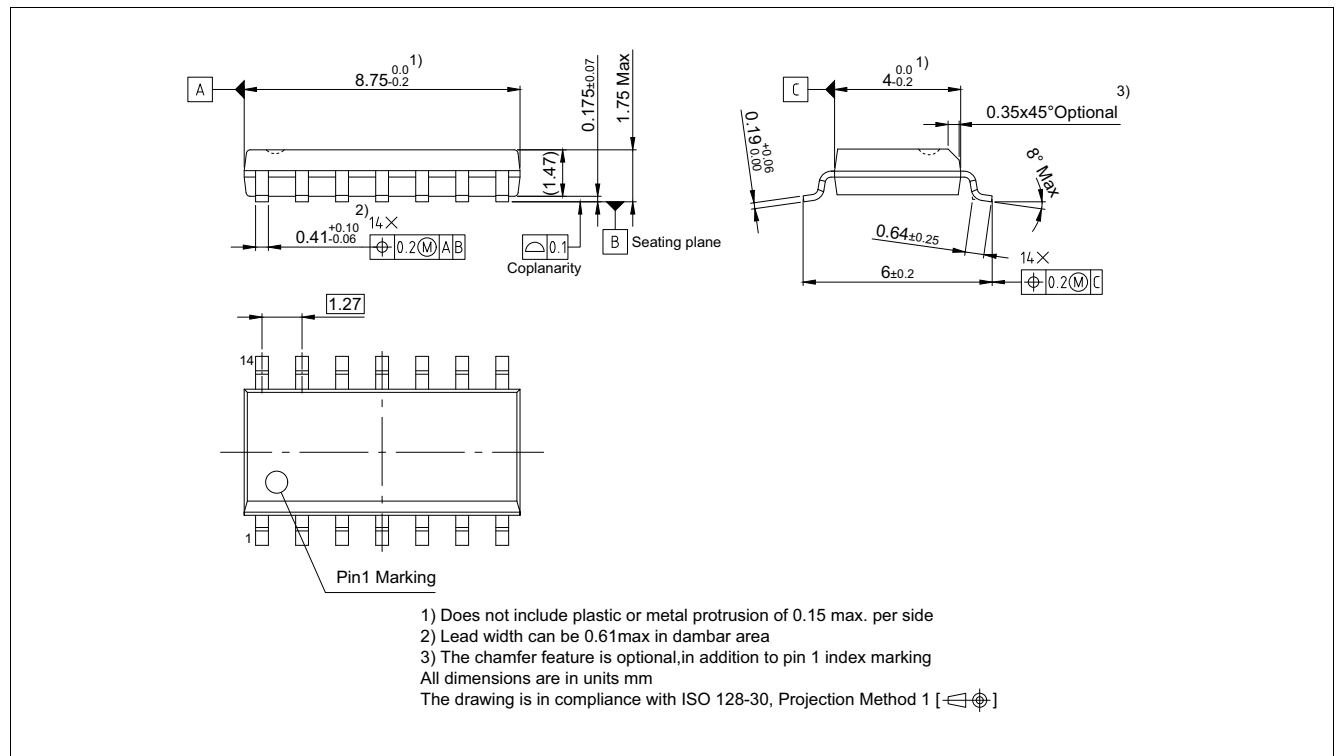
Figure 54 PG-DSO-14
