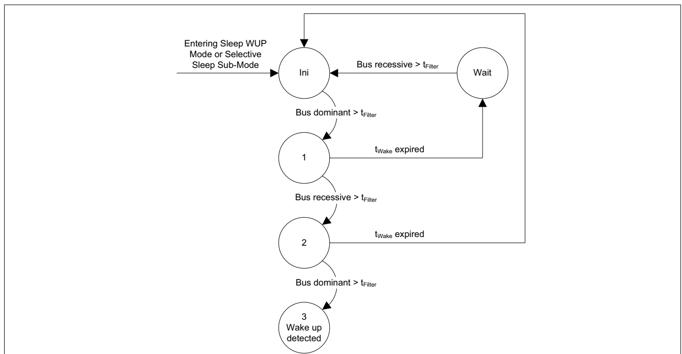
Figure 17 WUP detection
