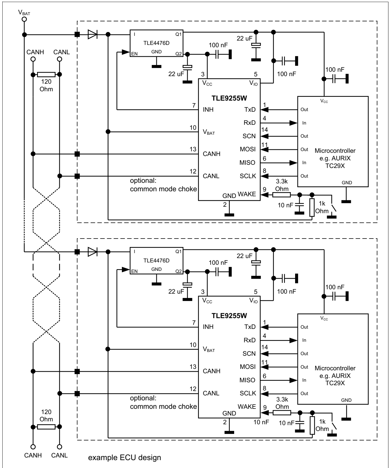
Figure 53 Application circuit
