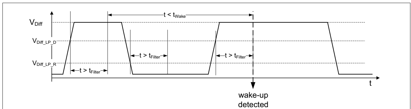
Figure 16 Wake-up pattern
