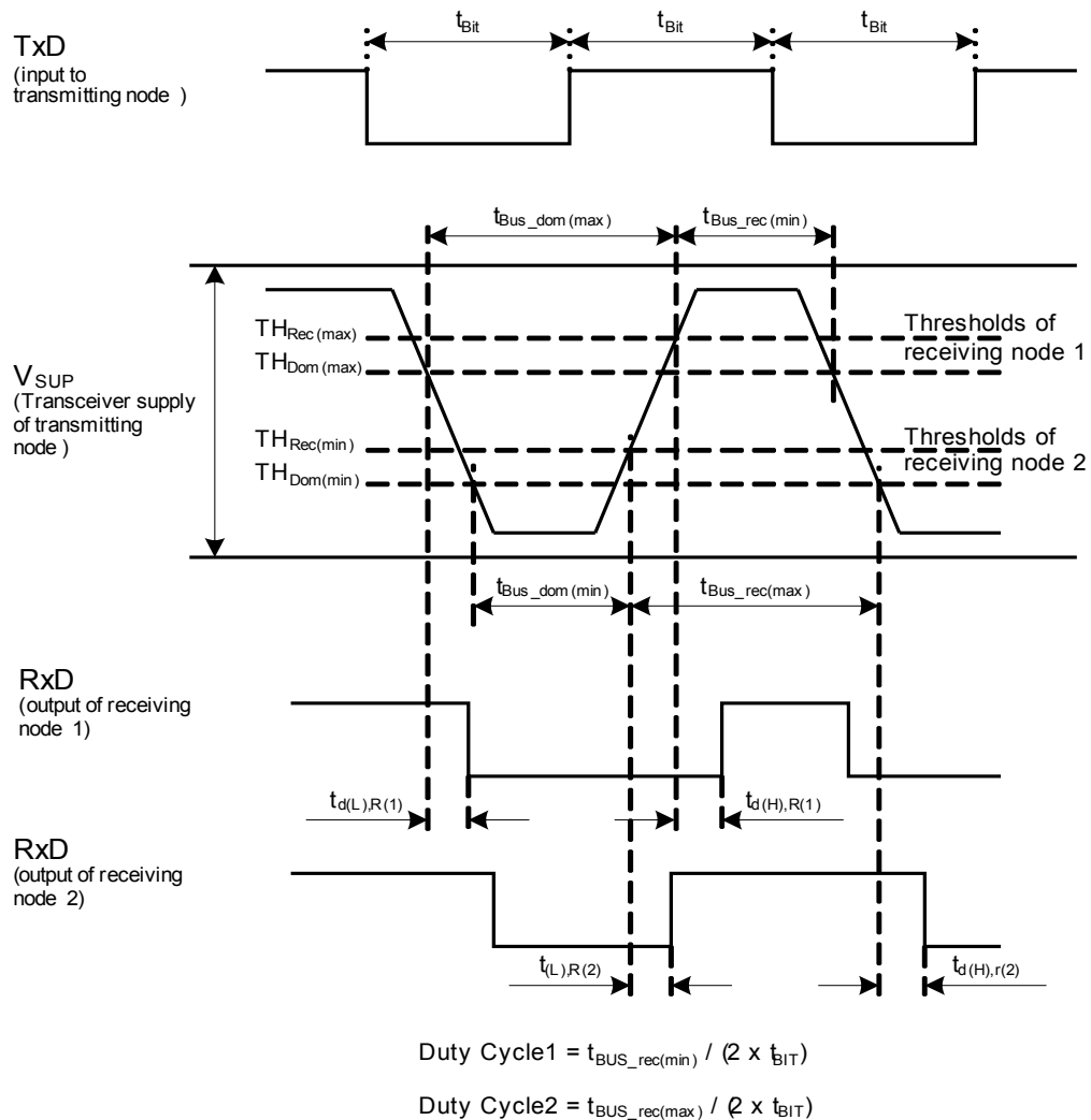
Figure 24 Timing Diagram for Dynamic Characteristics
