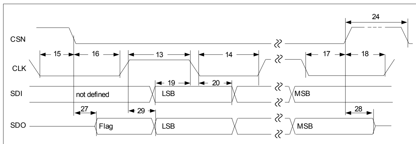
Figure 38 SPI Timing Diagram
