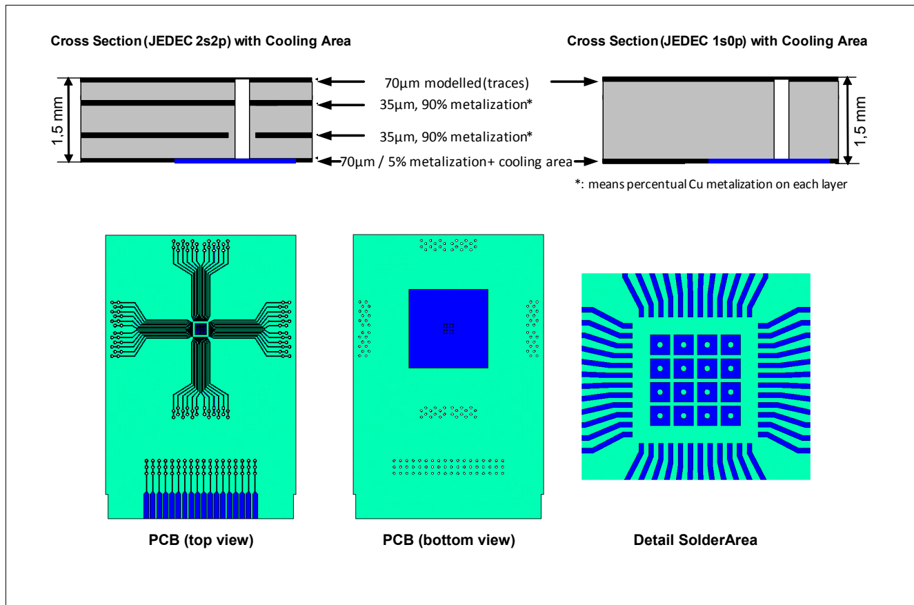
Figure 42 Board Setup
