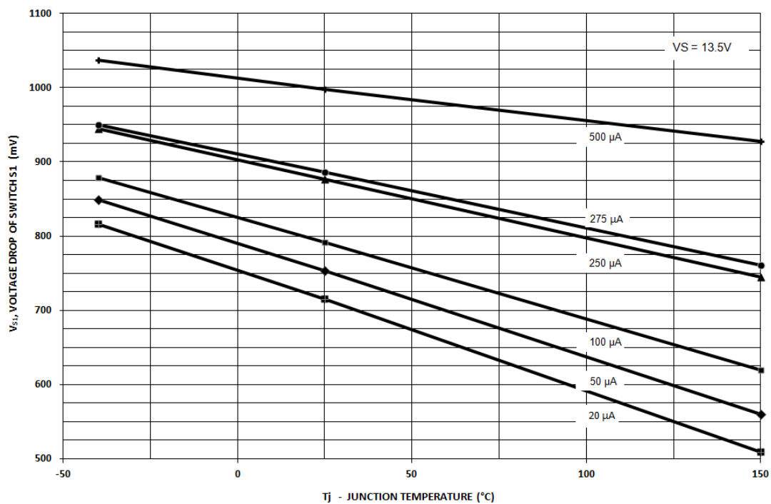
Figure 26 Typical Characteristics of S1 Drop Voltage (between WK1 & WK2) vs. Temperature for different S1 currents
