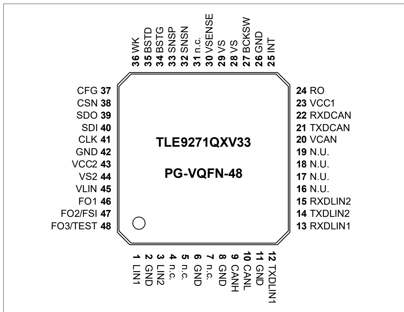
Figure 2 Pin Configuration
