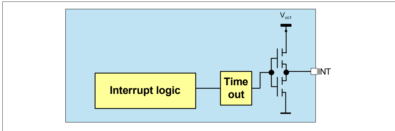
Figure 32 Interrupt Block Diagram
