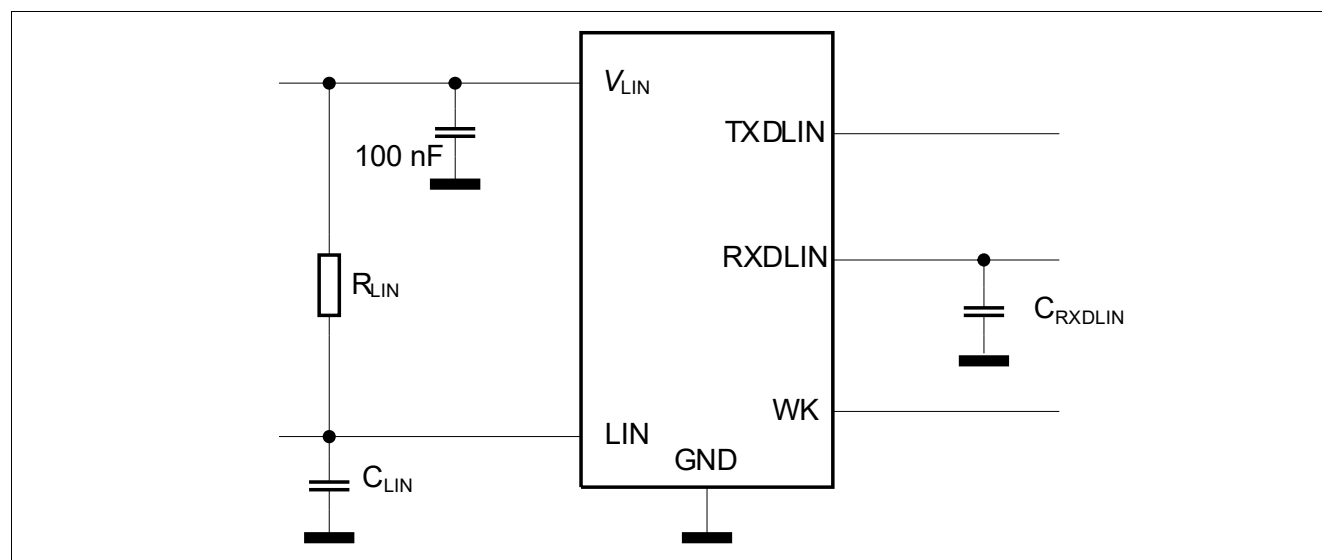
Figure 27 Simplified Test Circuit for Dynamic Characteristics
