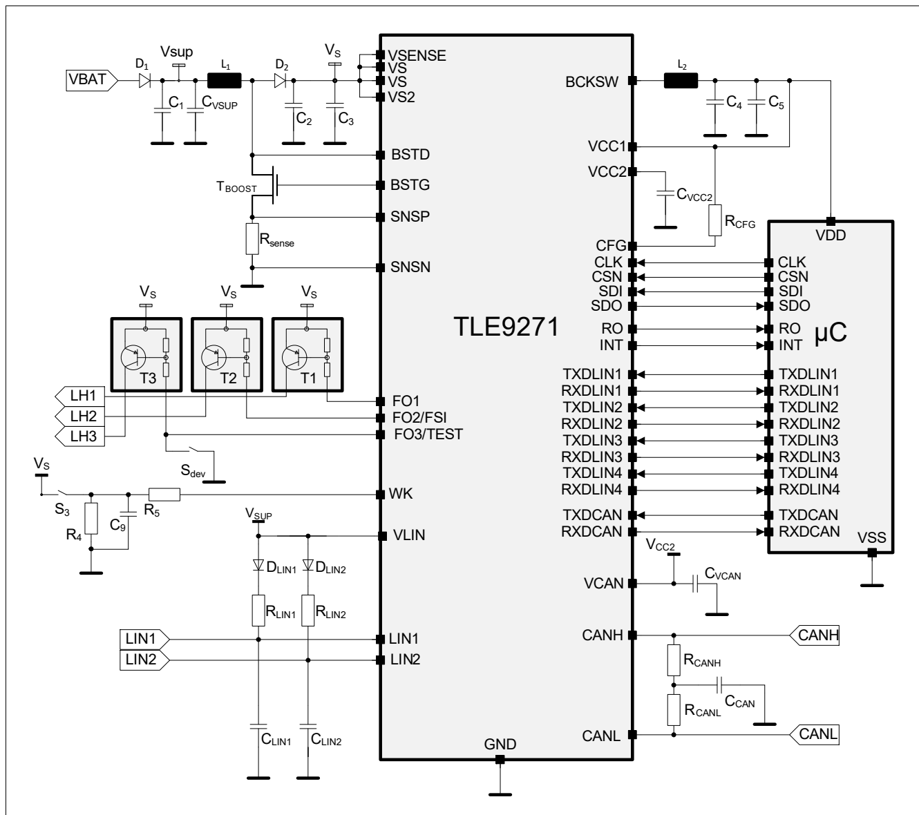
Figure 50 Application Diagram
