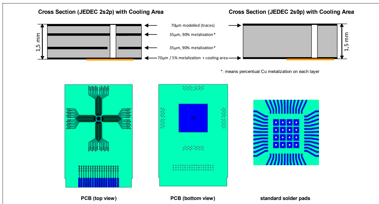
Figure 54 Board Setup
