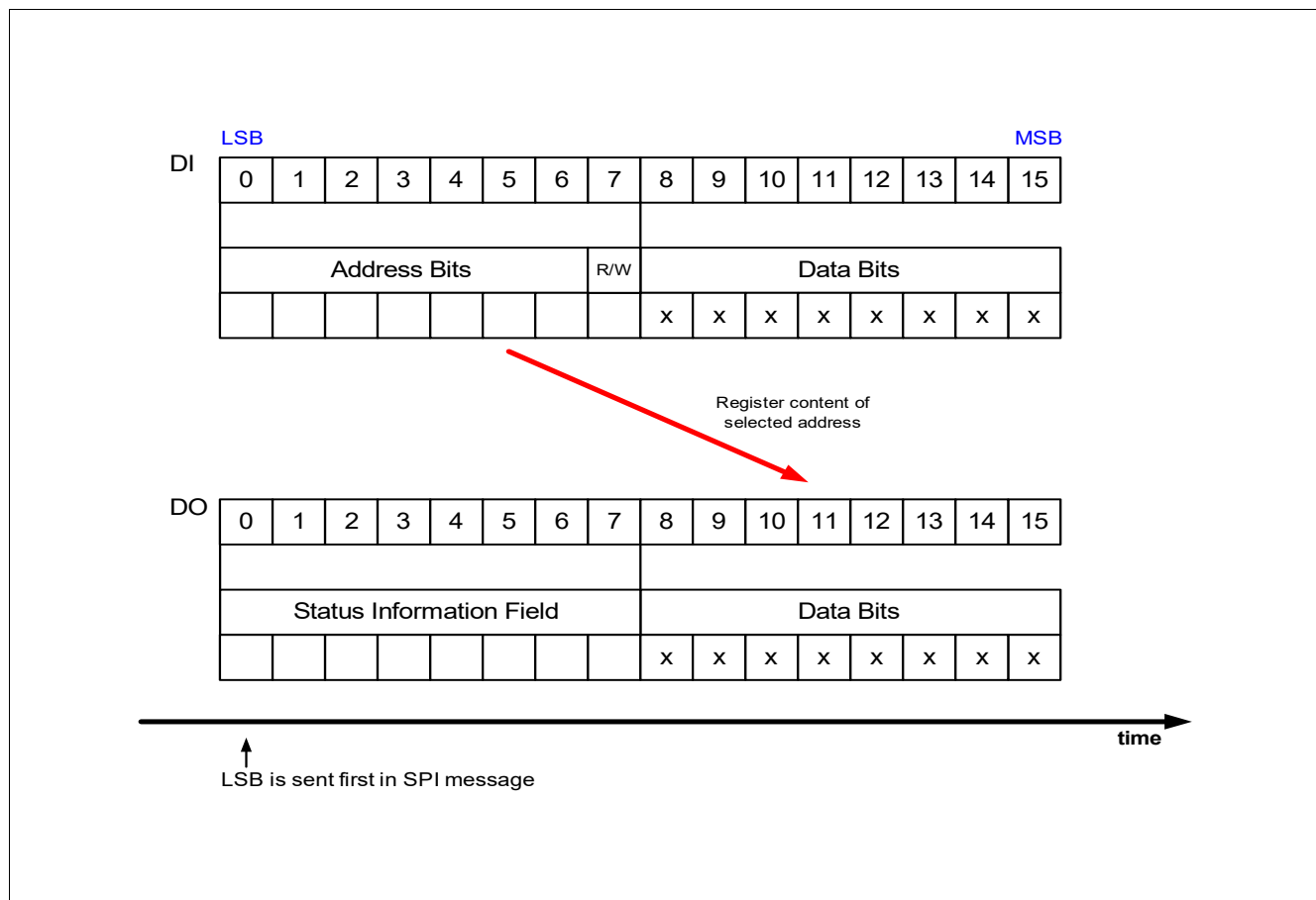
Figure 46 SPI Operation Mode
