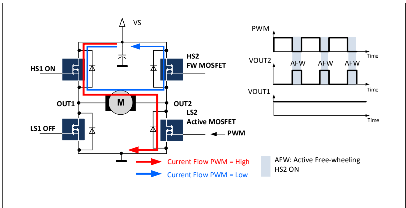
Figure 48 Active freewheeling on HB2: AFW2 = 1, HB2_PWM_EN = 1. PWM applied to LS2 (HB2MODE[1:0] = 01 B ). The motor operates as load: LS2 is the active MOSFET, HS2 is the FW MOSFET.
