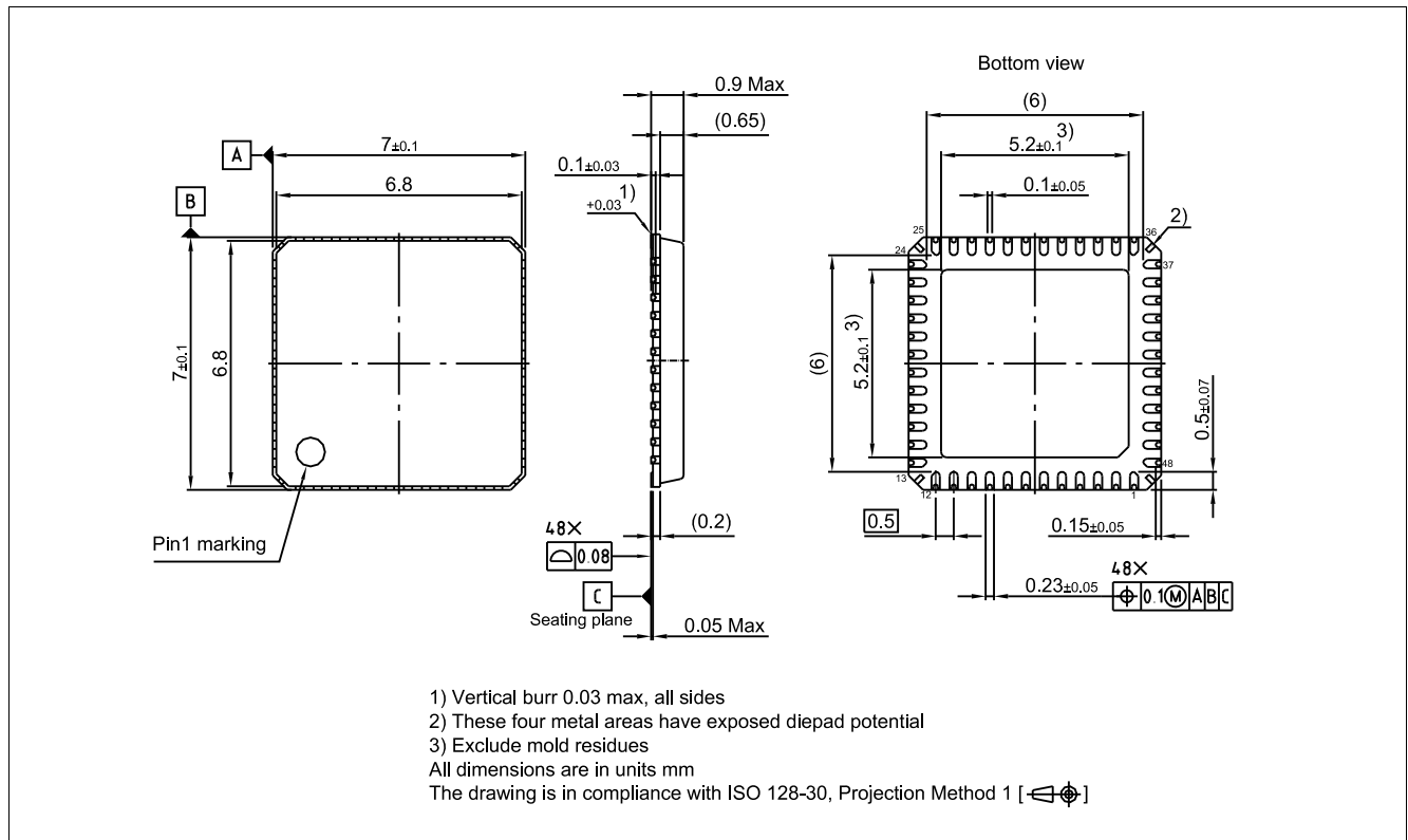
Figure 92 PG-VQFN-48-31
