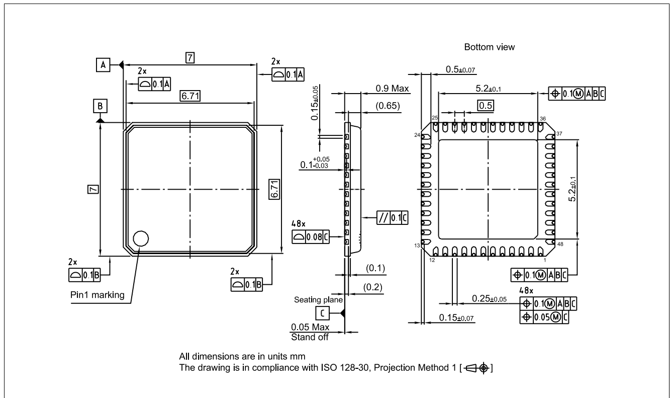
Figure 93 PG-VQFN-48-79
