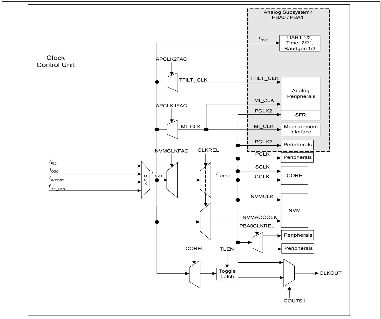
Figure 13 Clock Generation from f_{\text{sys}} ; CLKOUT Generation
