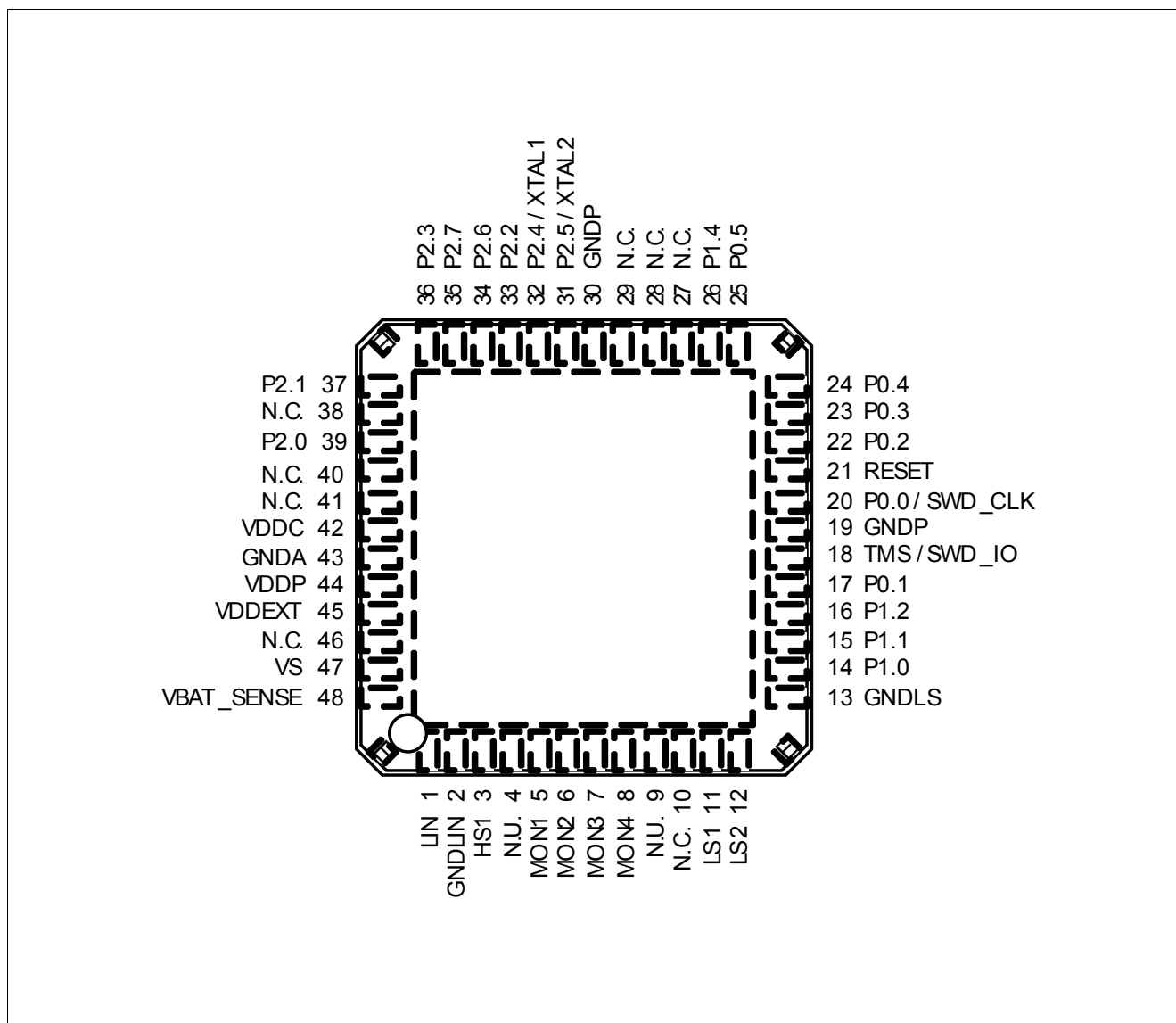
Figure 2 Device Pinout, TLE9844QX
