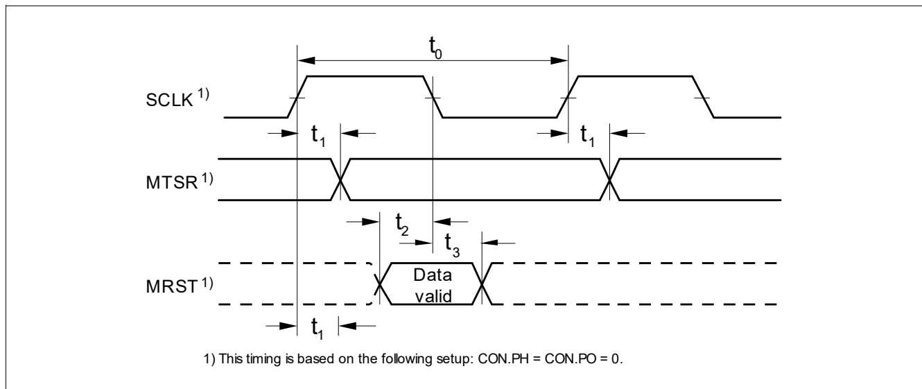
Figure 38 SSC master mode timing
