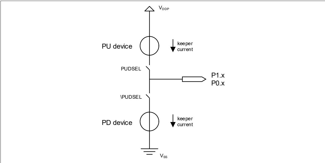
Figure 36 Pull-up/down device
