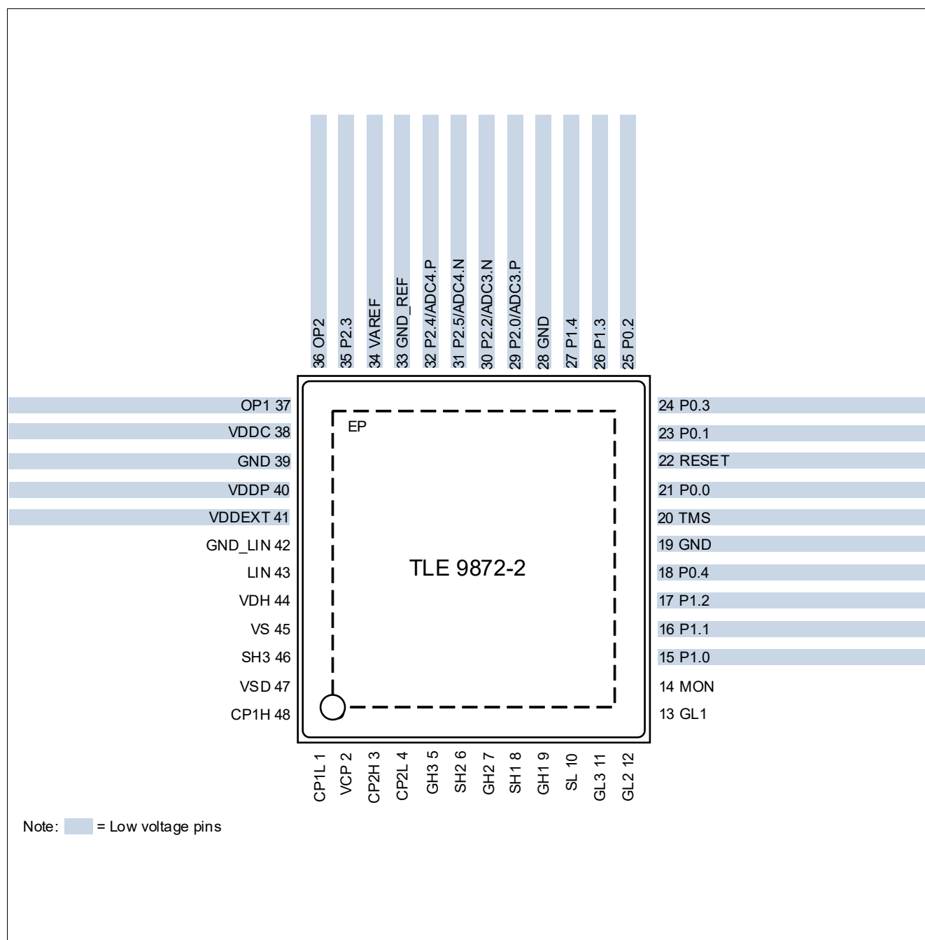
Figure 2 Device pinout
