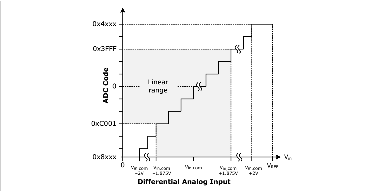
Figure 30 SDADC output code over input voltage
