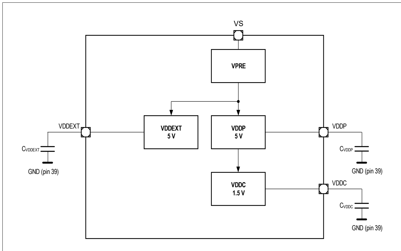
Figure 32 Load-sharing scenario for the VPRES regulator
