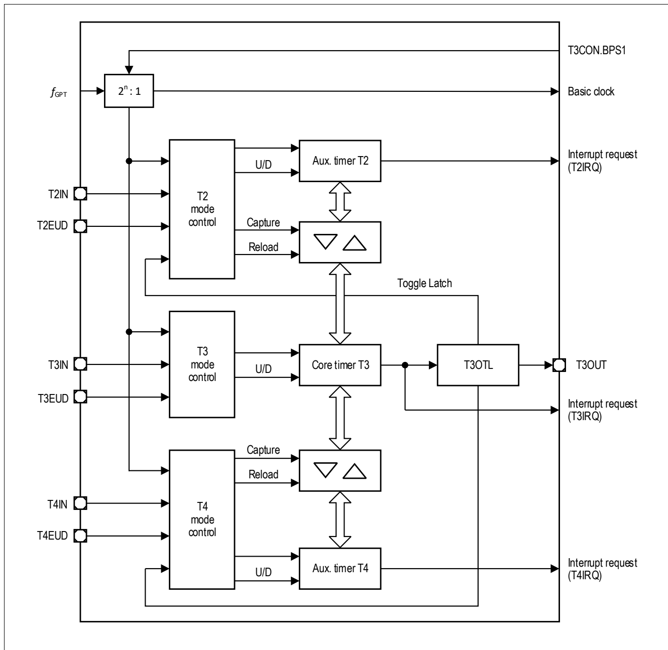
Figure 18 GPT1 block diagram ( n = 2 \dots 5 )
