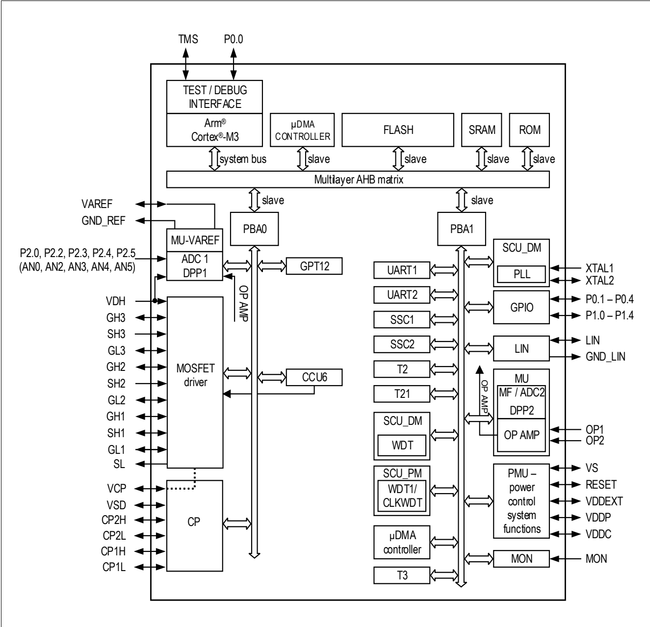
Figure 1 Block diagram
