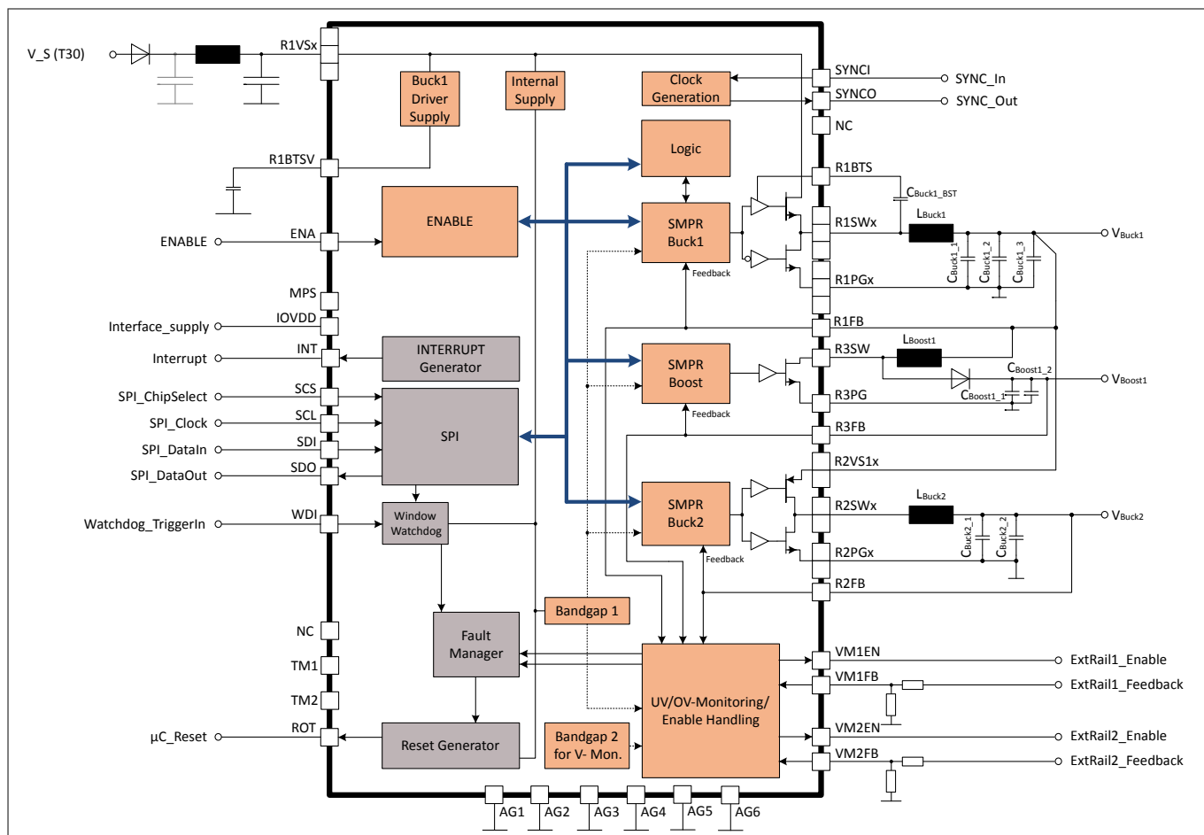
Figure 24 Application diagram
