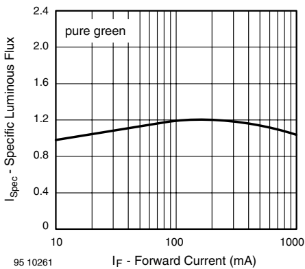
95 10261 I_F - Forward Current (mA) Figure 27. Specific Luminous Intensity vs. Forward Current
