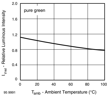
95 9991 T_{amb} - Ambient Temperature (°C) Figure 26. Rel. Luminous Intensity vs. Ambient Temperature
