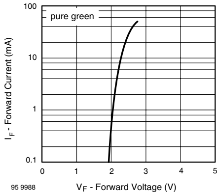
95 9988 V_F - Forward Voltage (V) Figure 25. Forward Current vs. Forward Voltage
