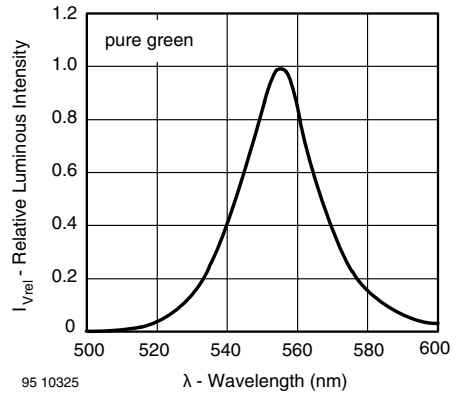
95 10325 \lambda - Wavelength (nm) Figure 29. Relative Intensity vs. Wavelength
