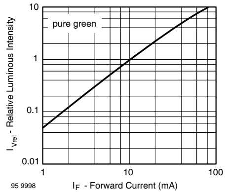
95 9998 I_F - Forward Current (mA) Figure 28. Relative Luminous Intensity vs. Forward Current
