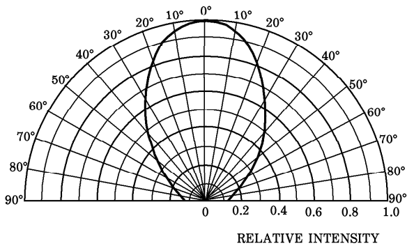
COUPLING CHARACTERISTIC WITH TPS613
