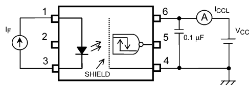
Fig. 13.1.3 I_{CCL} Test Circuit
